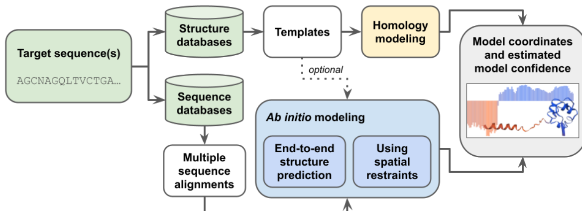
Figure 1. Schematic representation of modeling methods using target sequence(s), structure databases (e.g., PDB), and sequence databases (e.g., Uniclust30 [51]) as input to produce CSMs and estimates of prediction confidence. Homology modeling uses specific templates as its main input, while ab initio methods work without templates. Commonly used ab initio methods rely on multiple sequence alignments, which are either used directly as input for end-to-end structure prediction or processed to extract spatial restraints used to generate CSMs.
