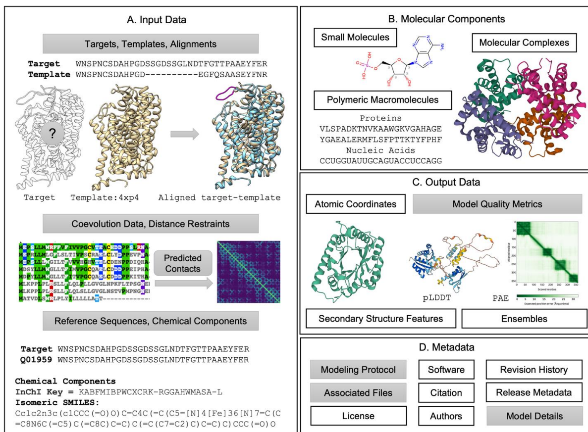
Figure 2. Schematic representation of the data specifications in ModelCIF. Definitions reused from PDBx/mmCIF are shown in white boxes (e.g., Atomic Coordinates) and the newly added definitions are shown in gray boxes (e.g., Model Quality Metrics). (A) Descriptions are provided for input data used in template-based and template-free modeling. (B) Representations of molecular components are retained from PDBx/mmCIF. (C) Definitions for atomic coordinates, secondary structure features, and ensembles are taken from PDBx/mmCIF; descriptions of local and global CSM quality metrics are defined in ModelCIF. (D) Several metadata definitions from PDBx/mmCIF are reused. New metadata definitions regarding modeling protocol, CSM classification ( ab initio , homology, etc.) and descriptions of associated files are included in ModelCIF. Examples of CSM-specific data and metadata represented in ModelCIF are provided in the Supplementary Material.
