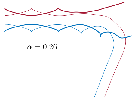
Fig. 2. Two perturbed leapfrogging orbits, the left one stable, the right one unstable.
