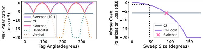
(a) Polarization Loss vs Tag Angle (b) Worst-Case Loss vs Sweep Size Fig. 3: Polarization Loss Simulations. a) Simulation results of polarization loss when sweeping with 10^\circ granularity (purple), switched (pink), horizontal (green), vertical (brown), and CP (gray). b) Simulation results of worst-case polarization loss vs sweep size (purple) compared to CP (gray) and switched polarization (pink x). Dotted lines denote loss at 45^\circ granularity.
