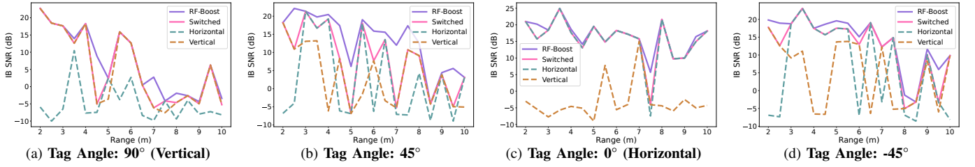
Fig. 5: In-Band SNR vs Range. IB SNR vs range for RF-Boost(purple), Vertical(brown), Horizontal(green), Switched(pink) with tags at a)90°b)45°c)0°d)-45°
