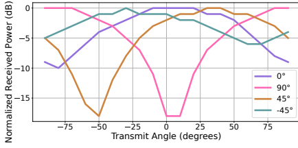
Fig. 6: Received Power vs Transmit Angle: Received power vs TX angle for an LP receiver at 0°(purple), 90°(pink), 45°(brown), and -45°(green)
