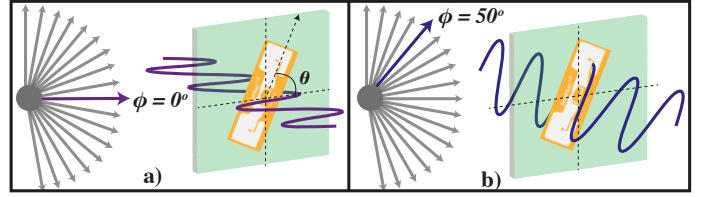
Fig. 2: Transmit Polarization Sweep. Two examples of transmit angles from a sweep of different angles. a) The transmitted angle has large polarization loss with the tag. b) The transmitted angle aligns well with the RFID.
