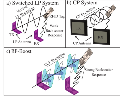
Fig. 1: RF-Boost . The majority of existing RFID readers leverage a) switched LP or b) CP antennas to read RFID tags, which suffer from large polarization mismatch. c) RF-Boost uses complex-controlled polarization to construct LP signals at various angles to minimize polarization loss.
