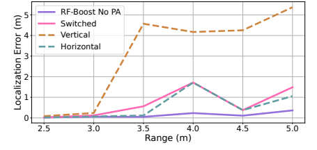
Fig. 8: Localization Error vs Range. Localization error vs range for RF-Boost-No PA(purple), Switched(pink), Vertical(brown), Horizontal(green)
