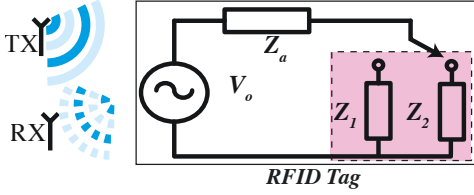
Fig. 4: RFID Tag Circuit. Thevenin equivalent circuit of an RFID tag showing the antenna impedance and the impedance of the two different states.
