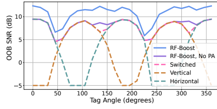
Fig. 7: OOB SNR. OOB SNR vs Tag Angle for RF-Boost(blue), RF-Boost-No PA(purple), Switched(pink), Vertical(brown), Horizontal(green)
