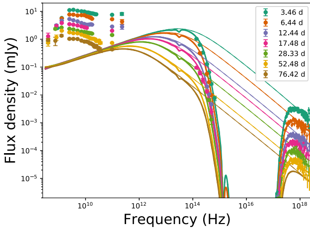
Figure 4. Multipepoch SEDs from our uGMRT, VLA, ALMA, NOEMA, and SMA programs, compared with optical observations and Swift/XRT SEDs at similar times, together with a wind FS model (lines). The FS cannot explain the observed radio flux and slowly evolving radio peak.
