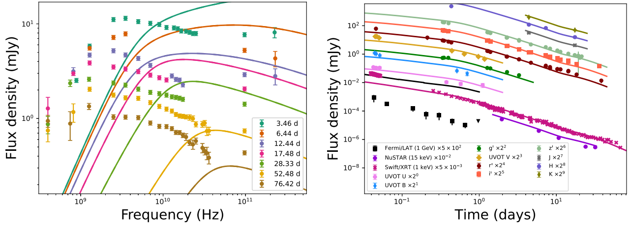
Figure 10. Radio SEDs (left) and light curves (right) for a low- p ISM model with parameters p = 1.5 , \epsilon_c = 0.07 , \epsilon_B = 0.03 , n_0 = 10 \text{ cm}^{-3} , E_{K,iso} = 1.5 \times 10^{52} \text{ erg} , and A_{V,host} = 0.3 \text{ mag} . This model requires a jet break at t_{jet} = 0.55 \text{ days} (implying \theta_{jet} = 9^\circ and E_K = 2 \times 10^{50} \text{ erg} ) in order to match the X-ray and optical light curves; however, the model significantly overpredicts the millimeter-band observations at \lesssim 28 \text{ days} , overpredicts the Fermi/LAT observations by two orders of magnitude, and does not match the centimeter-band SED at all, and is therefore ruled out.
