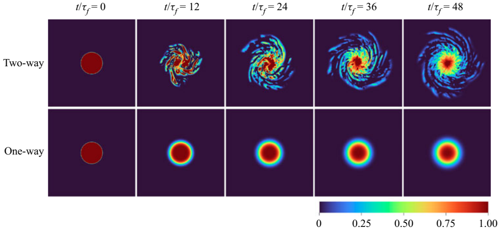
Figure 1. Isocontours of normalized vorticity ( \omega_z/\omega_c ) with St_\Gamma = 0.025 and Re_\Gamma = 1000 , for one-way coupling and two-way coupling at five non-dimensional times t/\tau_f .
