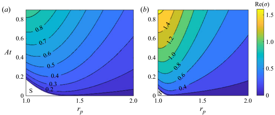
Figure 4. Contours of the analytically obtained growth rate (3.30) in the At - r_p plane for a Rankine vortex with St_r = 0 : (a) m = 2 ; (b) m = 4 .
