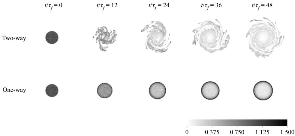
Figure 2. Isocontours of normalized particle volume fraction ( \phi_p / \langle \phi_p \rangle ) with St_\Gamma = 0.025 and Re_\Gamma = 1000 , for one-way coupling and two-way coupling at five non-dimensional times t/\tau_f .
