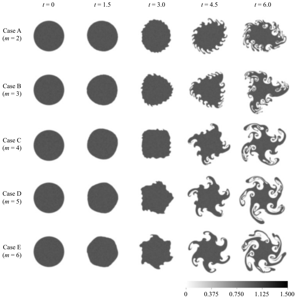
Figure 8. Isocontours of normalized particle volume fraction (\phi_p / \langle \phi_p \rangle) for cases A, B, C, D, E (see table 1 ) at five time instants. As time progresses, the inertial particles are expelled out of the vortex cores, forming cluster arms of which the number equals to the mode number. The small perturbations continue growing and ultimately destroy the structure.
