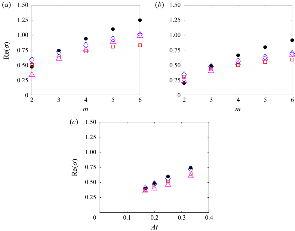
Figure 12. Comparison of instability growth rates between LSA and Eulerian–Lagrangian (EL) simulations at St_I = 0.002 and Re_I = 5000 . (a) Growth rates for mode numbers m = 2–6 at At = 1/3 ( M = 1 ). (b) Growth rates for mode numbers m = 2–6 at At = 1/5 ( M = 1/2 ). (c) Growth rates for mode m = 3 at various Atwood numbers. Symbols: ●, LSA; ◇, EL peak growth rate of the total perturbation energy; □, EL average growth rate of the total perturbation energy; △, EL peak growth rate of the seeded mode.
