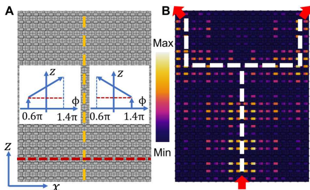
Fig. 5. Topologically protected surface wave splitter. (A) The schematic of surface wave pumping system and the corresponding phase modulation functions. (B) The magnitude of total displacement field distribution of the surface wave splitter. The surface wave is injected at the center of the bottom edge at the frequency f = 41.88 kHz.
