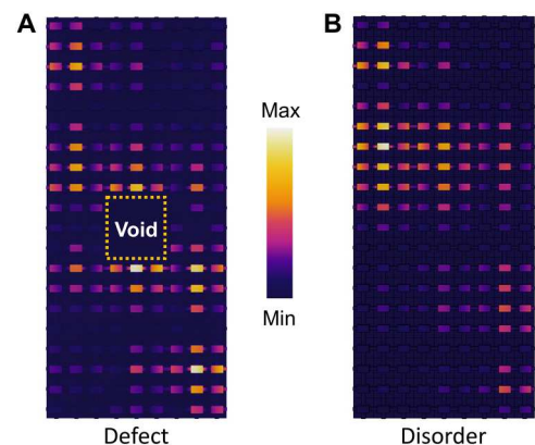
Fig. 4. Robust topological surface wave pumping. (A) The eigenmode of the defective structure at 41.75 kHz. The defect is constructed by removing 3 by 3 pillars in the dotted line box (B) The eigenmode of the disordered structure where a random normal distribution of errors is added on all geometric parameters at 41.88 kHz.
