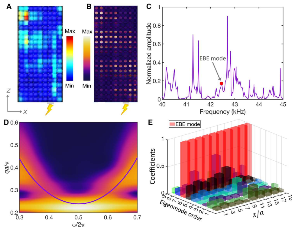
Fig. 2. Topological surface pumping on the elastic surface with space modulated pillars. (A and B) Experimental (A) and numerical (B) modal profile of the magnitude of the y directional (out-of-plane) displacement field at the frequencies f = 42.45 kHz and f = 41.88 kHz, respectively, by a piezoelectric patch (gray part in the bottom of the cuboid) excitation. (C) Frequency spectrum of the resonator with indices i = 2 and j = 18 from experimental measurement. The resonance peak noted by red dot is the EBE mode. (D) The wavelet transform of the eigenmode from numerical simulation along synthetic dimension. The purple curve is the interaction curve from Fig. 1D. (E) The mode decomposition of the displacement field in (B) of each chain for different z .
