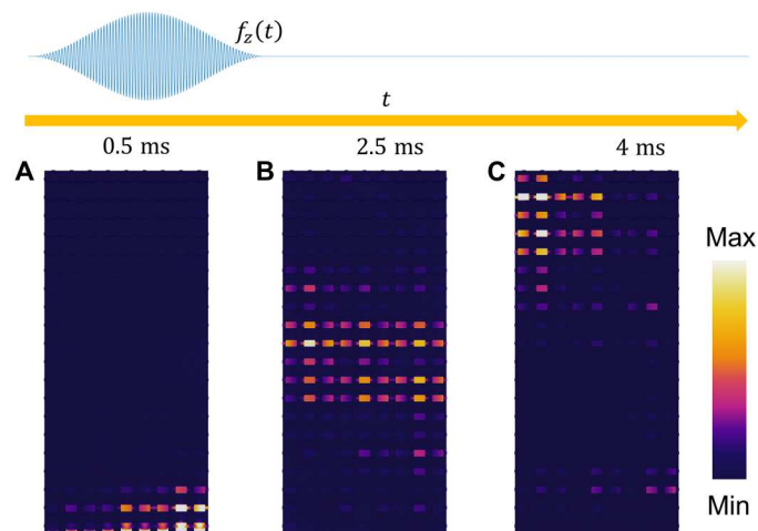
Fig. 3. Time response of the topological surface wave transport. (A to C). The magnitude of total displacement field at 0.5 ms, 2.5 ms, and 4 ms, respectively. A 50-cycle tone burst signal centered at 41.88 kHz is simulated on the bottom supercell.
