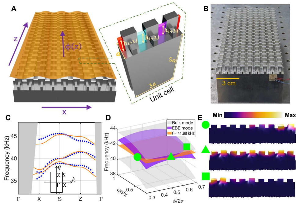
Fig. 1. Design principle and dispersion analysis. (A) Schematic illustration of the topological surface wave transport system. Each row in x corresponds to a supercell that includes three unit cells (inset). (B) Photograph of the experimental sample fabricated out of aluminum by a milling machine. The piezoelectric actuator on the bottom right serves as the excitation. (C) Numerically obtained dispersion curves (blue dots) for the unit cell with \phi_j = \pi . The orange curves represent the dispersion curves of the discrete mass-spring model obtained by numerical fitting. The gray regions are filled with bulk modes. Their interfaces with the surface wave region define the sound cone. (D) Dispersion diagram for the supercell terminated by free boundary conditions in the x direction and Floquet boundary conditions in the z direction. The edge-bulk-edge (EBE) mode is represented by the magenta surface, whereas the bulk bands are indicated by gray surfaces. The orange cut plane corresponds to the excitation frequency f_c = 41.88 kHz. The interaction curve between excitation frequency plane and EBE surface gives the instantaneous wave number q(z) on which the circle is right edge mode, the triangle is the bulk mode, and the square is the left edge mode. (E) The top, middle, and bottom panels are the corresponding eigenmodes of supercell at \phi = 0.6\pi (circle), \pi (triangle), and 1.4\pi (square) with q = \pi/a in (D).
