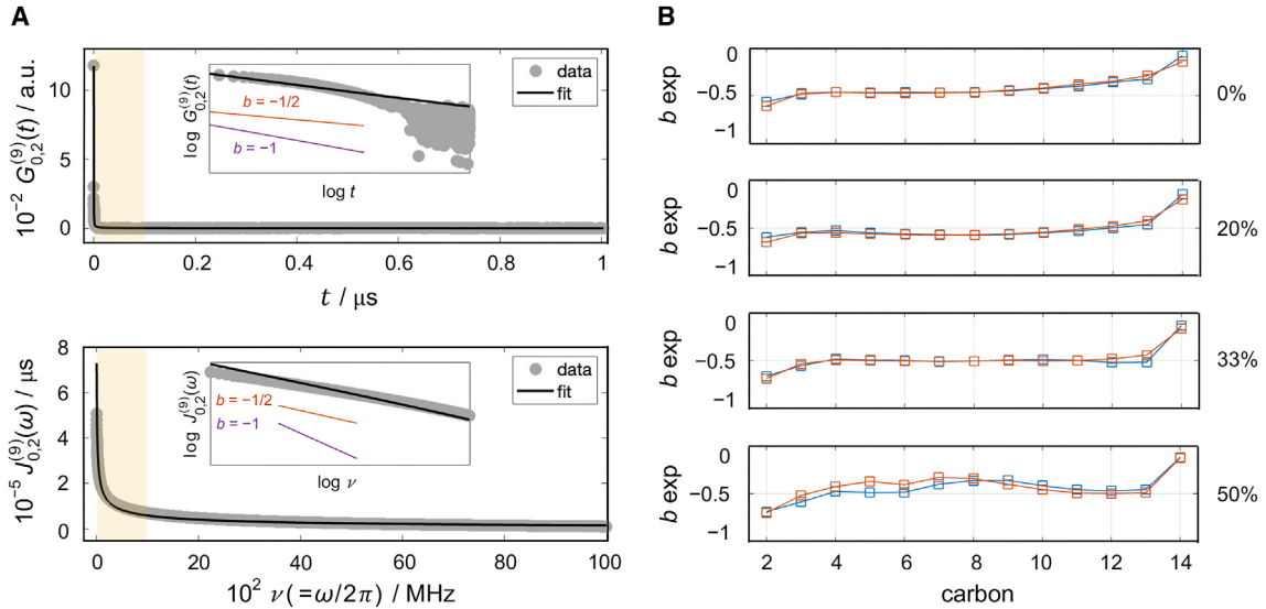
FIGURE 2 Illustration of dynamics of CH bond fluctuations. (A) Example of (top) autocorrelation function G_{0,2}^{(9)}(t) and (bottom) spectral density J_{0,2}^{(9)}(\omega) for carbon C9 of the sn -2 chain of DMPC. The results correspond to fluctuations of the CH bonds as described by the Wigner D_{00}^{(2)}(\Omega) function. Simulation data are shown in gray and best power-law fit to the simulation results in black. Insets show expansion of the data from the highlighted region from 0 to 1000 MHz but in a log-log plot. Shown for comparison are sample functions of the form ax^{-1} (purple) and ax^{-1/2} (red). (B) Power exponents of best fits to the spectral densities J_{0,s}^{(n)}(\omega) for carbons C2–C14 on the sn -1 (red) and sn -2 (blue) chains of DMPC with 0, 20, 33, and 50 mol % cholesterol. The power exponents of all carbons in all simulated bilayers are close to -1/2 , consistent with collective segmental dynamics. All simulations were performed at 44°C. See text for details. To see this figure in color, go online.
