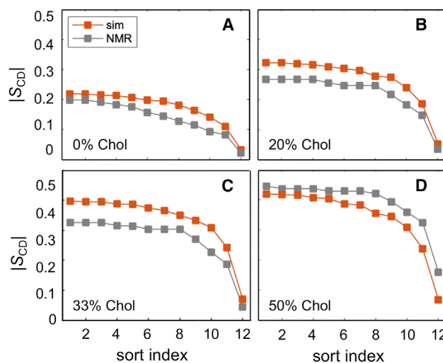
FIGURE 10 Comparison of DMPC order profiles obtained from simulations and NMR spectroscopy. Acyl chain order parameters are shown for DMPC bilayers containing (A) 0 mol %, (B) 20 mol %, (C) 33 mol %, and (D) 50 mol % cholesterol. The results are plotted as a function of sort index (i.e., in descending order) either calculated from simulations (red) or reported from NMR (gray). Simulation data are average from the two chains. Experimental data were taken from (34) with the 0 mol % cholesterol values interpolated from the data at 30°C, 50°C, and 60°C. All simulations were performed at 44°C. Validation of lipid force fields with NMR data requires consideration of both order parameters and relaxation rates. See text for details. To see this figure in color, go online.
