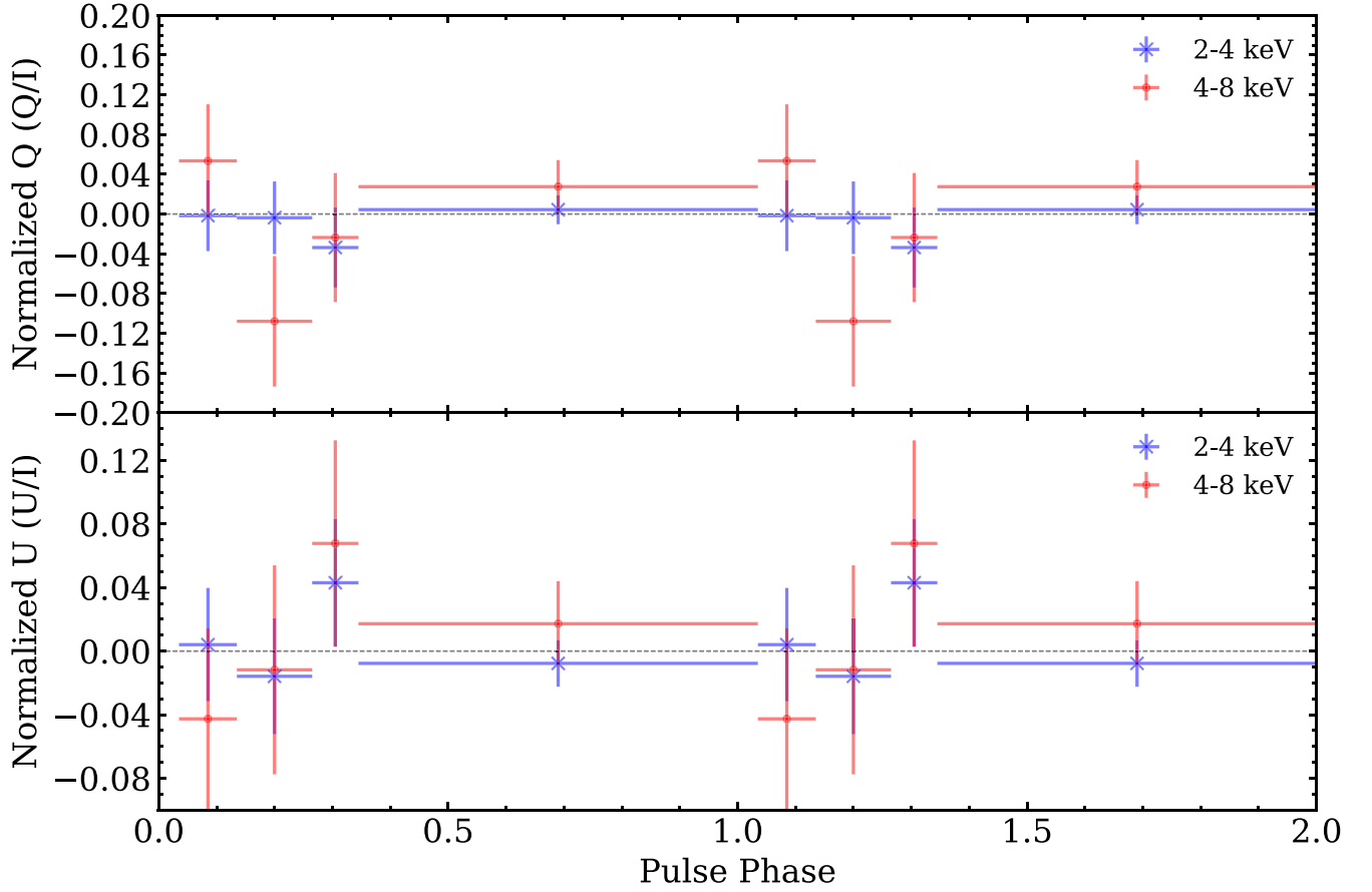
Figure 5. Normalized Q ( Q/I ; top) and normalized U ( U/I ; bottom) as a function of pulse phase in the 2–4 keV (blue) and 4–8 keV (red) energy bands. Two rotation cycles are plotted for clarity. The error bars denote 1\sigma uncertainties for one degree of freedom. There is no clear detection of polarized emission in either energy band for any phase interval.
