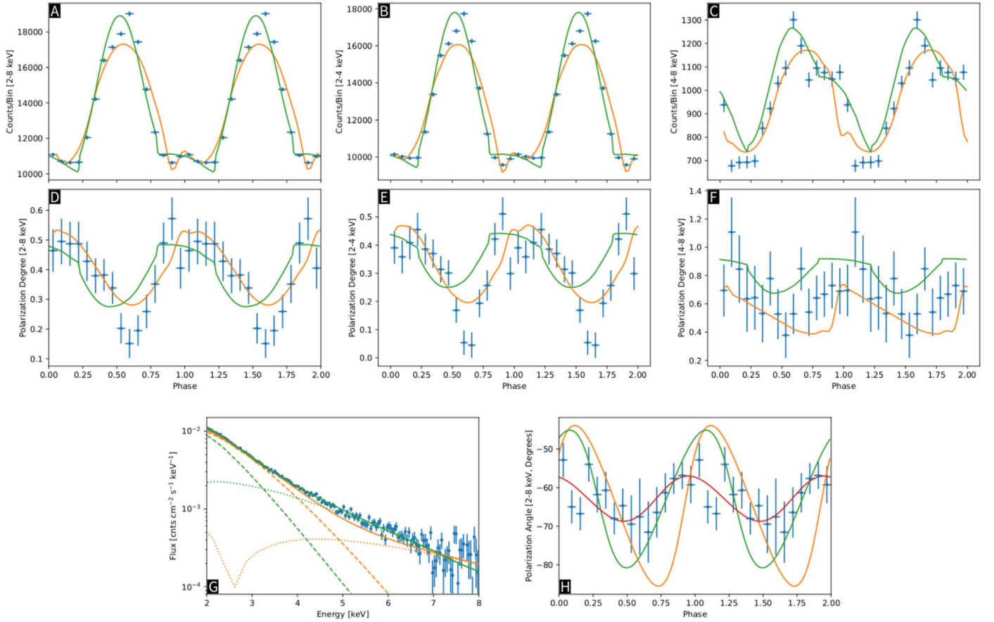
Figure 4. 1RXS J1708 IXPE observation (blue circles with error bars) for the source counts (panels (A)–(C)) and polarization degree (panels (D)–(F)), plotted as a function of the rotational phase (in each row, the three panels from the left to the right show the data integrated over the 2–8, 2–4, and 4–8 keV bands, respectively). Panels (G) and (H) show: (left) the phase averaged spectrum (solid lines) together with the contributions of the condensed zone (dashed lines) and atmospheric zone (dotted lines); (right) the polarization angle as a function of the rotational phase, integrated over the 2–8 keV band. Errors are shown at the 1\sigma level assuming the polarization degree and polarization angle are not correlated. In all panels, the orange and green lines represent the model expectation within the belt+cap and cap+cap scenarios (solid lines for the total model, dotted and dashed lines in panel (G) only for the two separate components); the red solid line in panel (H) shows the RVM (see the text for the parameter values and other details). Note that data points in the phase-resolved analysis are obtained with IXPEOBSSIM, and therefore independent on the spectral decomposition.
