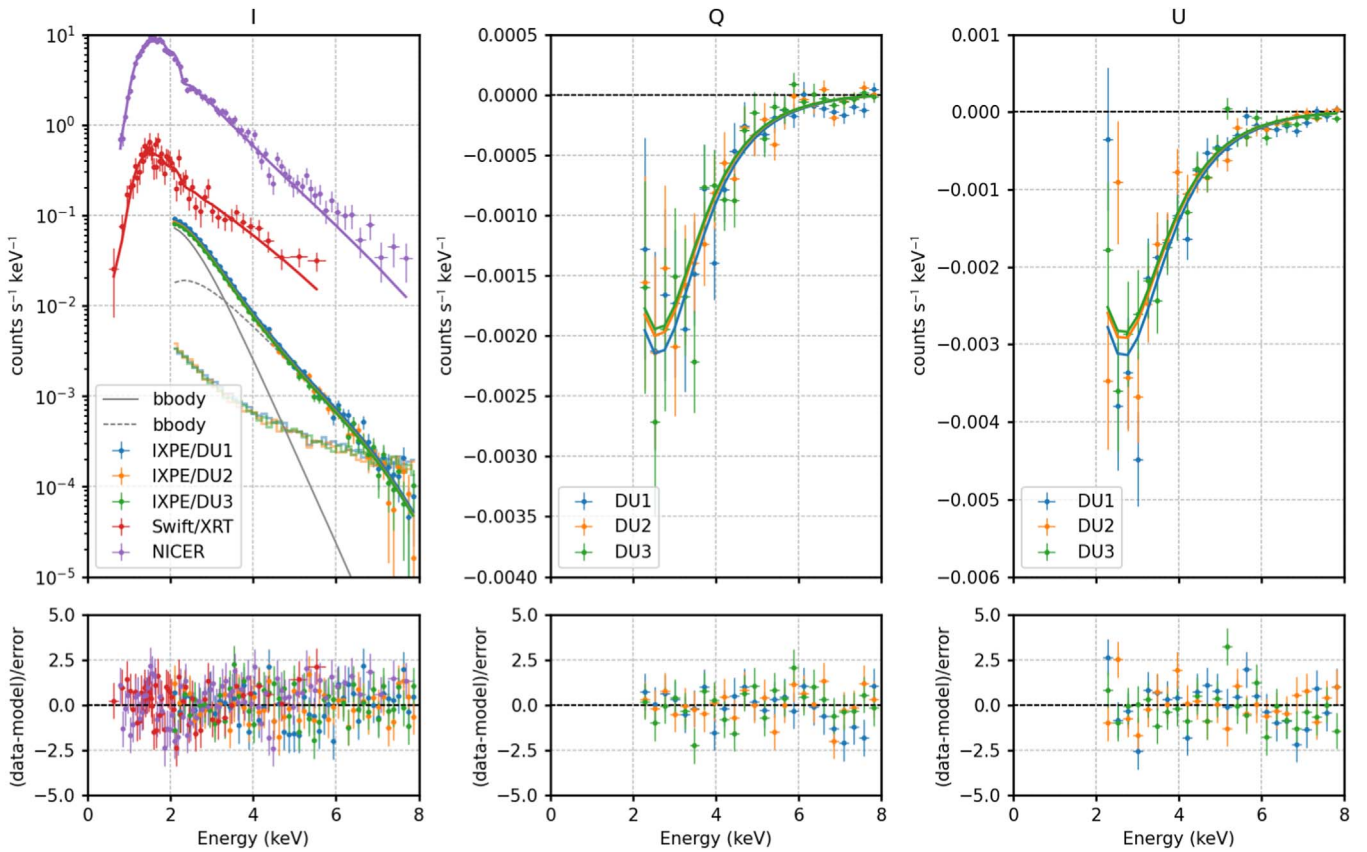
Figure 3. Same as in Figure 2, for the TBABS*(BBODY * POLCONST + BBODY * POLCONST) model. See Table 2 in Appendix B for the fit parameters.
