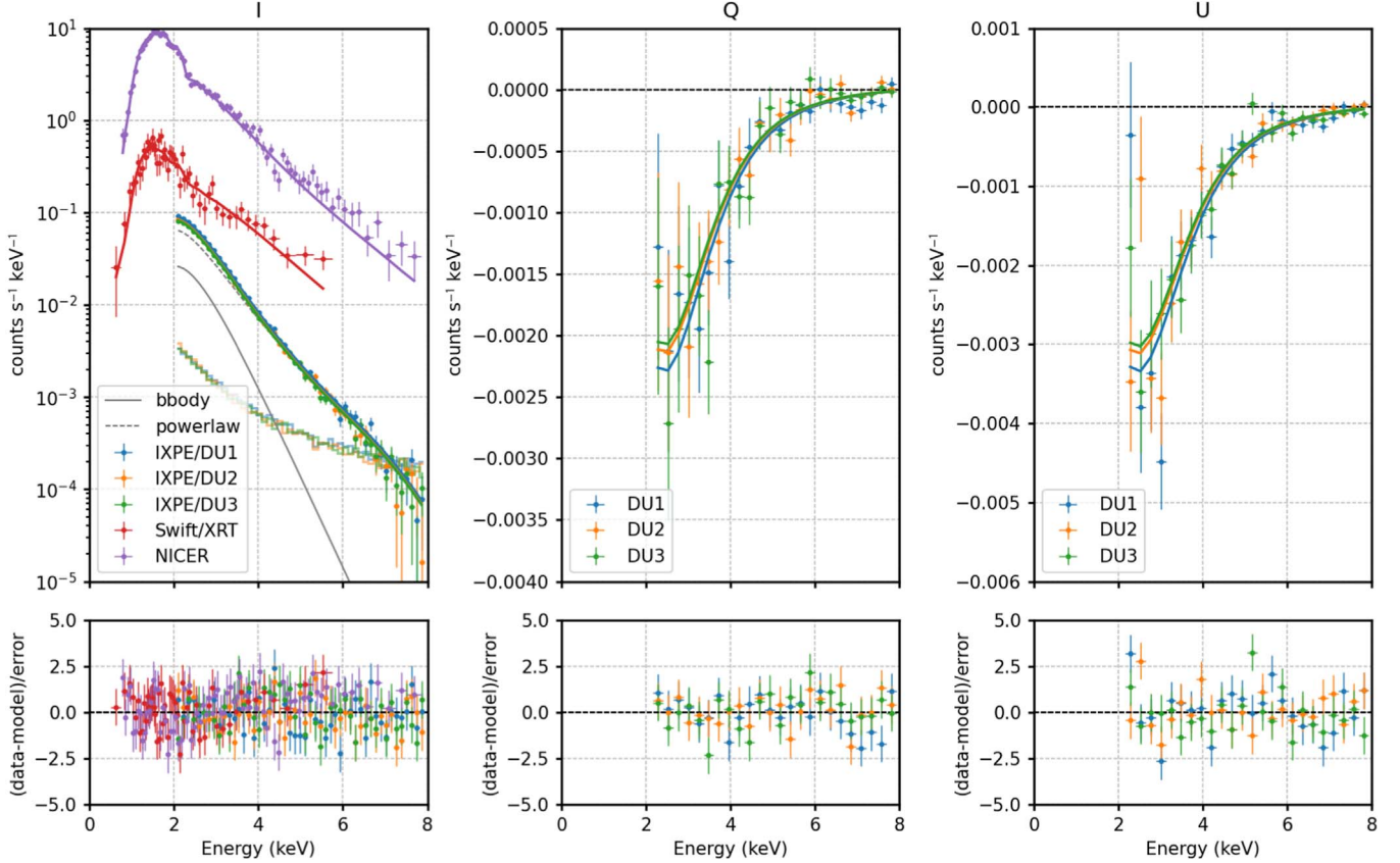
Figure 2. Joint spectropolarimetric fit of IXPE, Swift/XRT, and NICER data. The Stokes I , Q , and U energy spectra are obtained by binning the event-by-event Stokes parameters, calculated following Kislak et al. (2015), according to the measured energy of the event. Q and U are given by the source flux multiplied by the polarization degree and either the cosine or the sine of twice the polarization angle, respectively. The Stokes I , Q , and U energy spectra convolved with the instrument response are shown in the left, central, and right panels, respectively. The best-fit model of the form \text{TBABS}^*(\text{BBODY} * \text{POLCONST} + \text{POWERLAW} * \text{POLCONST}) is shown by the solid lines. Fit residuals are shown in the bottom panels; see Table 2 in Appendix B for the fit parameters. Light colored curves are the background of IXPE detectors.
