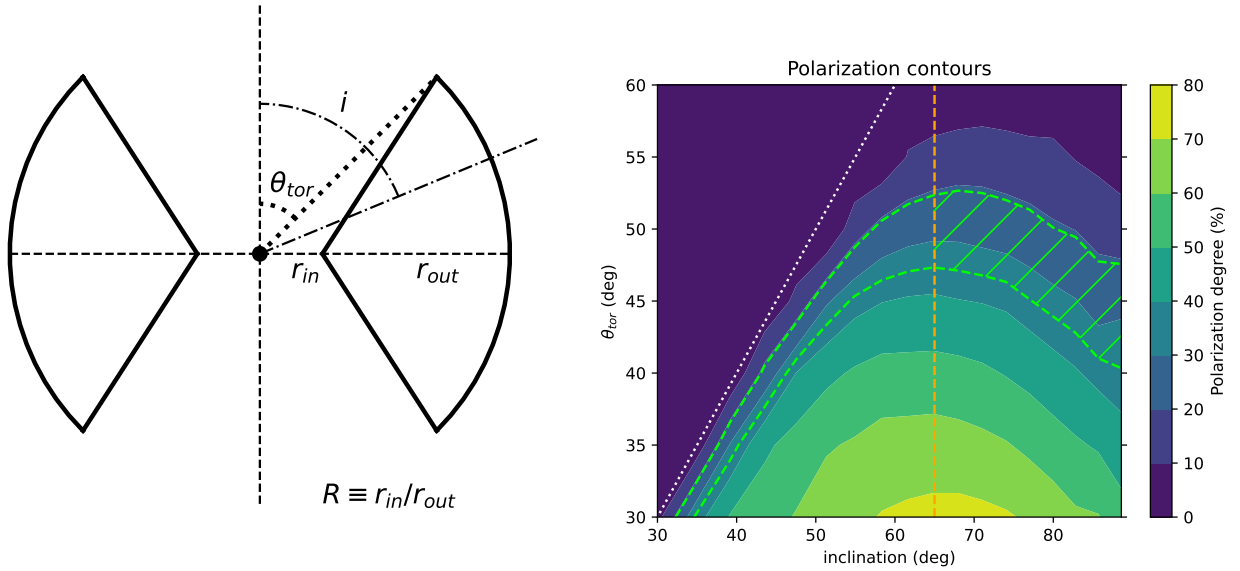
Figure 6. Left panel: Sketch of the torus geometry assumed for polarimetric modelling. The torus opening angle \theta_{tor} and the observer inclination i are both measured from the symmetry axis. Right panel: Contour plots of the constant polarization degree calculated for scattering off a torus, on the \theta_{tor} - i plane. The white dotted line corresponds to the equality \theta_{tor} = i ; the condition for the obscuration of the central source is \theta_{tor} < i . The green dashed curves enclose the 68 per cent confidence level region on the measured polarization for the cold reflector in the Circinus galaxy. The orange dashed line marks the inclination of the host galaxy, likely a lower limit to the torus inclination (as discussed in the text). The green hatches mark the region of the parameter space consistent with all the observational constraints.
