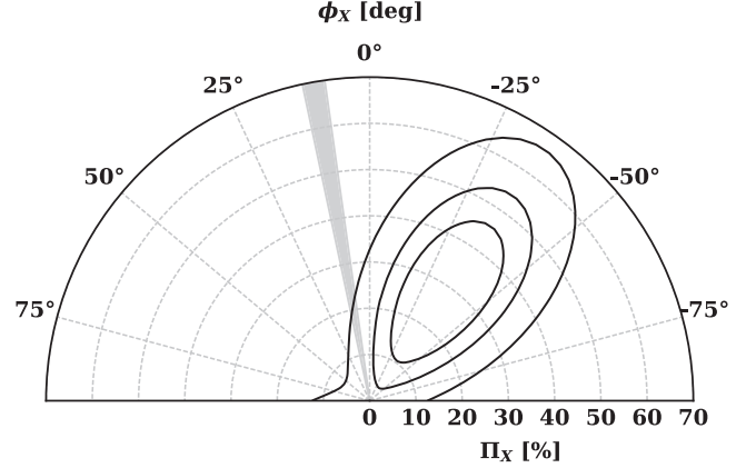
Figure 5. Polarization fraction and EVPA confidence levels (68%, 95%, 99%) for the low-energy power law in Figure 1. Gray shaded region represents the VLBI-determined jet axis projection on the plane of the sky (Weaver et al. 2022).
