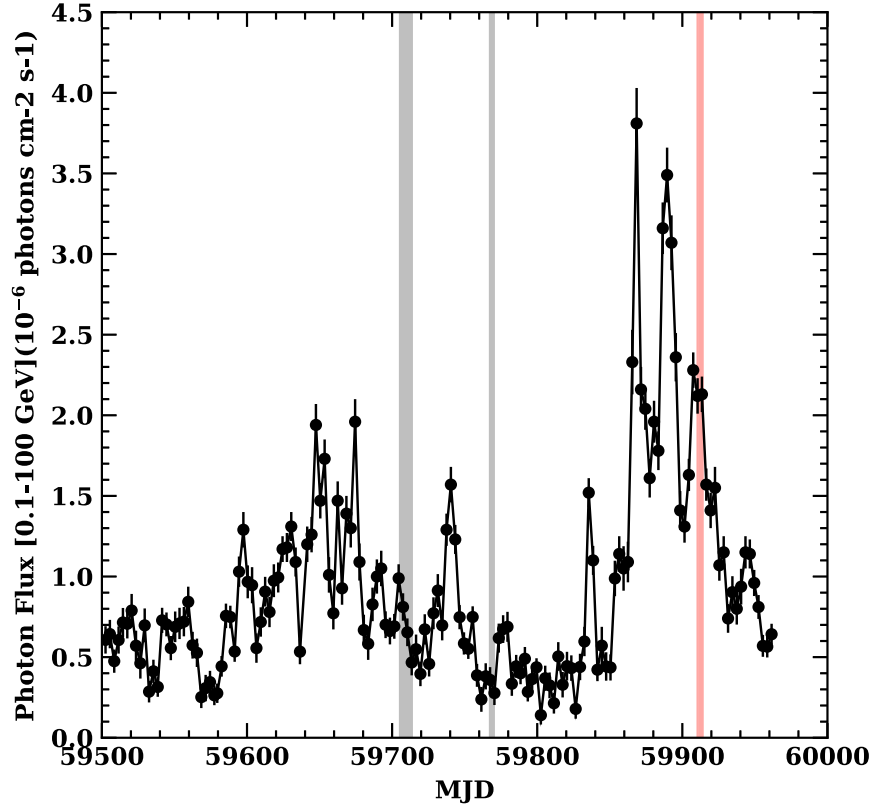
Figure 8. Fermi-LAT three day cadence light curve, showing the outburst that triggered the IXPE observation. A single power-law model with a free photon index is used to determine the photon fluxes. The two gray shaded regions demarcate two previous IXPE observations, while the red shaded area indicates the observation discussed in this paper.
