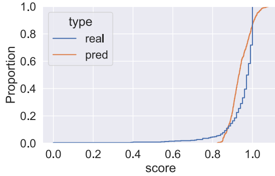
Fig. 11. CDF of Predicted Privacy Risk and Groundtruth
