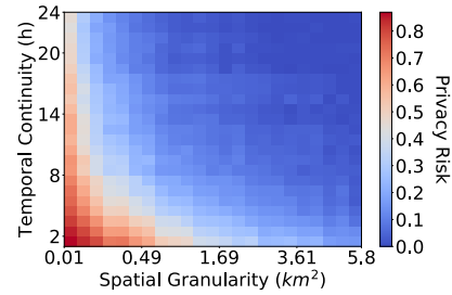
Fig. 2. Privacy Risk Contour for Vehicles with K = 4 (The spatial granularity denotes the area of a cell in a grid with a specific side, e.g., the area of a cell in 1km \times 1km grid is 1(km)^2 .)
