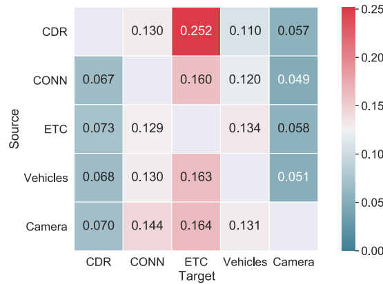
Fig. 10. RMSE Grid of TransRisk with K=2
