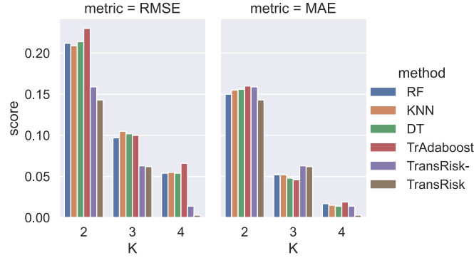
Fig. 7. Performance of One Week Data
