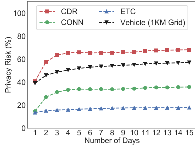
Fig. 1. Privacy Risk Evolution with K = 4 (The x-axis denotes the number of days of data is used for calculating the privacy risk, and the y-axis denotes the average user privacy risk of the users involved in the corresponding data.)
