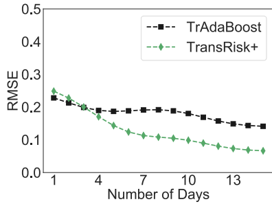
Fig. 13. RMSE of 3 Weeks
