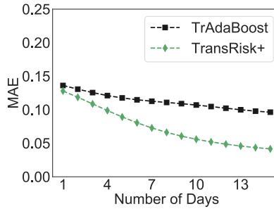
Fig. 14. MAE of 3 Weeks
