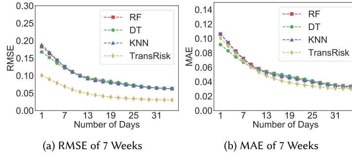
Fig. 8. RMSE and MASE of All Methods on 7 Weeks Data ( K=3 )
