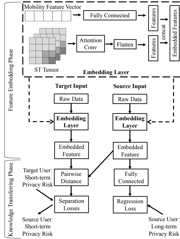
Fig. 4. Framework of TransRisk
