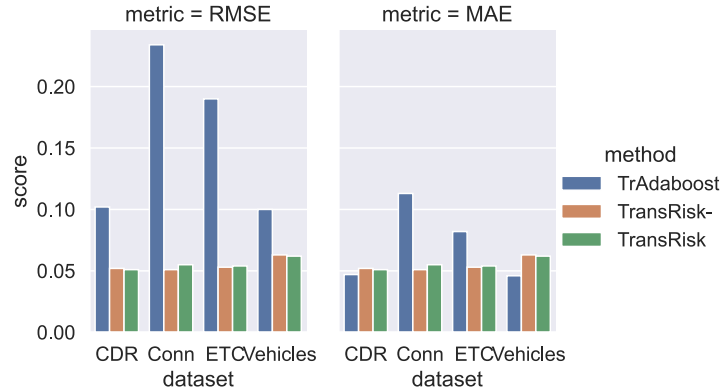
Fig. 9. Performance of Different Data Sources
