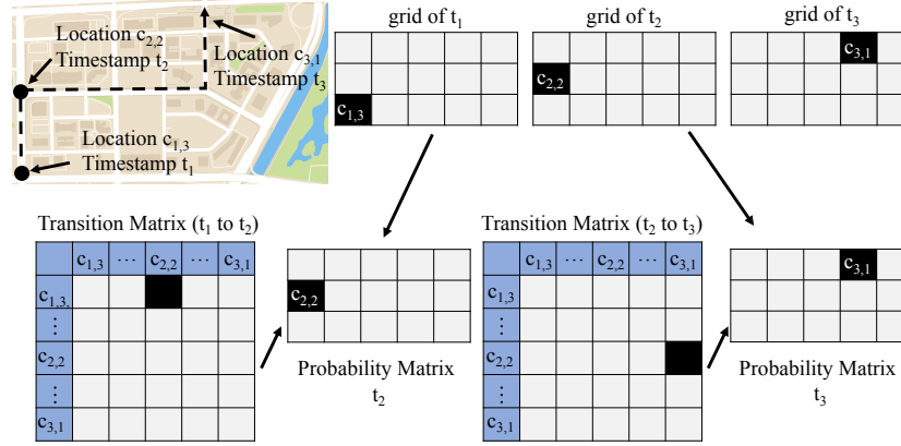
Fig. 5. Example of ST tensor
