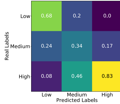
Fig. 12. Predicted Labels Grid
