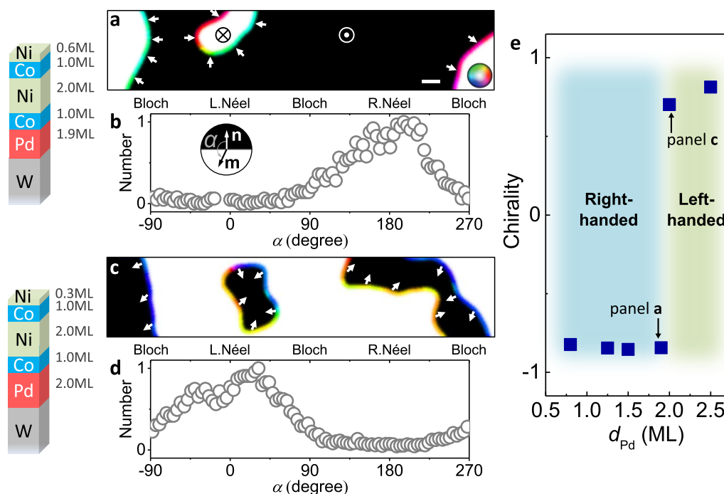
Figure 1. Tunable DMI system of (\text{Ni}/\text{Co})_2/\text{Pd}(d_{\text{Pd}})/\text{W}(110) with perpendicular magnetization. (a) Compound SPLEEM image at d_{\text{Pd}} = 1.9 ML. Black/white regions represent up/down domains (see symbols), and the color wheel shows the in-plane magnetization direction within domain walls (also highlighted by white arrows). Scale bar is 200 nm. (b) Histogram of angle \alpha between boundary normal vector \mathbf{n} and in-plane magnetization \mathbf{m} (see inset), measured pixel-by-pixel along domain boundaries, showing right-handed Néel-type chirality. (c) Compound SPLEEM image at d_{\text{Pd}} = 2.0 ML. (d) Histogram of angle \alpha , showing left-handed Néel-type chirality. (e) Chirality evolution as a function of d_{\text{Pd}} . Chirality is defined as (N_{\text{Left}} - N_{\text{Right}})/(N_{\text{Left}} + N_{\text{Right}}) , N_{\text{Left}} is the number of domain wall pixels where \alpha is between -90^\circ and 90^\circ , and N_{\text{Right}} is the number of domain wall pixels where \alpha is between 90^\circ and 270^\circ .
