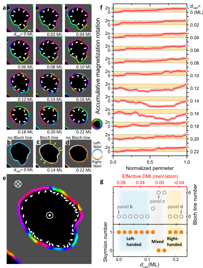
Figure 3. DMI-dependent evolution of skyrmion structures in (\text{Ni/Co})_2/\text{Pd}(2.05 \text{ ML})/\text{W}(110) capped by Pd. (a) Sequence of compound SPLEEM images with various Pd d_{\text{cap}} . Black/gray indicates up/down domains, and the color wheel highlights the in-plane magnetization direction on the skyrmion boundary (also shown by the white arrows). Scale bar is 200 nm. (b–d) Decomposed Néel-component images of the same area at d_{\text{cap}} = 0 , 0.14 and 0.22 ML. The blue, white, and orange color wheel highlights left-handed Néel-type, Bloch-type, and right-handed Néel-type domain wall segments, respectively. Yellow arrows in panel c indicate the positions of Bloch lines, where the Néel-type chirality are opposite on both sides. (e) Enlarged compound SPLEEM image for d_{\text{cap}} = 0.14 ML in panel a, highlighting the detailed magnetization rotation along the boundary (by white arrows), where the accumulative magnetization rotation is 0. (f) d_{\text{cap}} -dependent accumulative magnetization rotation around the perimeter of the skyrmion bubble, the counting starts from the bottom of the image with counterclockwise direction. The color-bar highlights the range of magnetization rotation for homochiral cases, where the rotation is expected to be monotonic between 0 and 2\pi . (g) Evolution of Bloch line number and skyrmion number as a function of d_{\text{cap}} (lower x-axis) and the effective DMI strength (upper x-axis). The Bloch line number represents the frequency of Néel-component switching within one skyrmion bubble, where the number 0 means fully chiral and a finite number indicates a mixed chirality.
