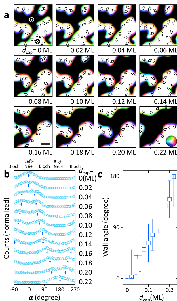
Figure 2. Chirality evolution of the Pd(capping)/(Ni/Co) 2 /Pd(2.05 ML)/W(110) as a function of Pd capping layer thickness, d_{\text{cap}} . (a) SPLEEM image sequence at varying Pd capping thicknesses. Black/white regions represent up/down domains, and the color wheel highlights the in-plane magnetization direction within domain walls (also shown by white arrows). Scale bar is 500 nm. (b) d_{\text{cap}} -dependent \alpha -histogram, indicating a gradual shift of the peaks (blue arrows). (c) Averaged domain wall angle with respect to the boundary's normal direction (from white to black) as a function of d_{\text{cap}} , showing a gradual transition.
