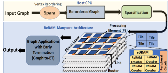
Fig 1: Schematic illustration of the GraphIte architecture.
