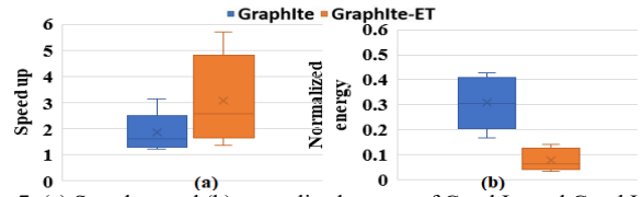
Fig. 7: (a) Speed up and (b) normalized energy of GraphIte and GraphIte-ET for PageRank with respect to Spara.
