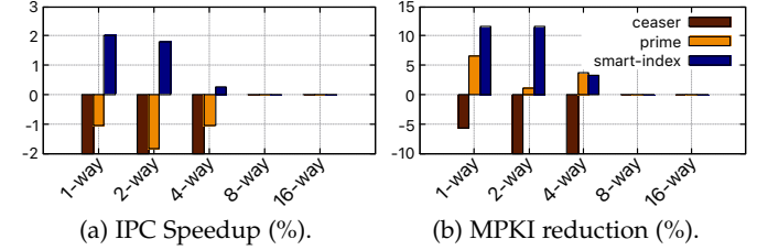
Fig. 5: Performance comparison between indexing techniques on different cache associativity for non-uniform applications. 1-way is direct mapped cache. 8/16-way columns are empty since there is no non-uniform application (Table 3).
