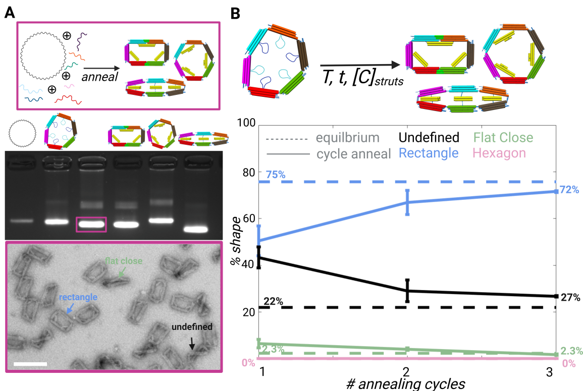
Figure 2(A) Schematic showing competitive folding of 6-bar with scaffold and all core and strut staples (top) Agarose gel electrophoresis image left to right: 7249 m13p18 scaffold, direct fold of 6-bar with no strut staples, competitive fold as shown in schematic above, direct fold of rectangle shape, direct fold of hexagon shape, and direct fold of flat close (middle) TEM image of competitive fold showing the preferred shapes (bottom) scale bar = 50nm (B) Schematic showing folded 6-bar open configuration added with strut strands and annealed to form a mixture of rectangle, hexagon, and flat close shapes (top) Plot of competitive fold of 6-bar compared to cycle annealing of folded 6-bar mechanism with strut staples; dotted line = equilibrium average, solid line = cycle annealing (bottom). CAD models visualized in UCSF Chimera 39 Created with BioRender.com
