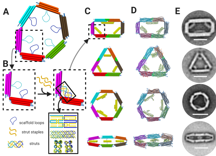
Figure 1: (A) 6-bar mechanism is comprised of six bars/arms connected by six hinges. Each arm contains a 172 nt scaffold loops protruding towards the middle of the mechanism. (B) The 172 nt scaffold loops can be combined and folded via addition of staple strands (yellow) to form struts, which are depicted schematically and in oxDNA 36–38 simulations (bottom of lower right inset). (C) CAD models with dsDNA helices depicted as cylinders and (D) oxDNA 36–38 simulations of the 6-bar mechanism showing four shapes: rectangle, triangle, hexagon, and flat-closed. (E) TEM image averages of each shape validating designs and simulations where each shape is formed by distinct strut configurations. Scale bars = 50nm. CAD models visualized in UCSF Chimera 39 . Schematics created with BioRender.com
