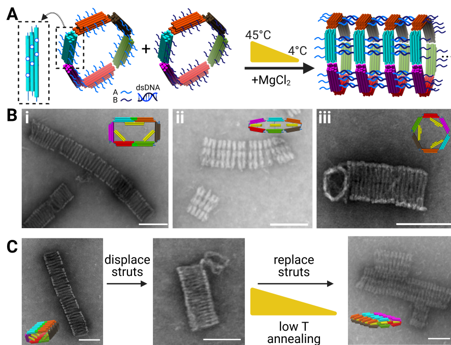
Figure 4: (A) left to right: Schematic showing polymerization scheme of the 6-bar tubes (inset showing in-plane location of polymerization strands on each arm) with each arm having 6 in-plane and 6 out-of-plane polymerization strands. Unit “A” and “B” polymerize via complementary sticky ends and subjected to a low temperature thermal annealing ramp to form tubes with distinct cross-sections. (B) TEM images of DNA origami tubes with (i) with rectangle cross-section (ii) flat-closed-cross section (iii) hexagon cross-section (insets are CAD models of each tubes cross-section shape) (C) Reconfiguration schematic of DNA origami tubes with TEM images (left) Rectangle cross-section (middle) rectangle cross-section subjected to displacement staples and incubation (right) Displaced tubes mixed with transformation strut staples to reconfigure to flat-closed cross-section. Scale bars = 100nm. CAD models visualized in UCSF Chimera 39 . Created with BioRender.com
