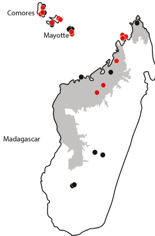
Figure 12. Distribution of Erromyrmex latinodis in the Malagasy region. Red indicates localities of sequenced specimens.
