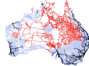
Figure 3: Power transmission lines (black), shown together with not accessible (red), and accessible (blue) routes of Australia by a 400 km ranged EV using existed charging stations. The coloring method is described in the caption of Figure 2.
