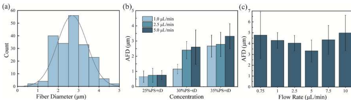
Fig. 4 (a) Histogram of fiber diameter distribution of electrospun fibers prepared with PS solution concentration of 35 wt % at a flow rate of 1.0 \mu\text{L min}^{-1} . Average fiber diameter of the SMP electrospun fibers with different PS solution concentrations at various flow rates, (b) tD/PS (25, 30, and 35 wt %), and (c) tD/PS (40 wt %).
