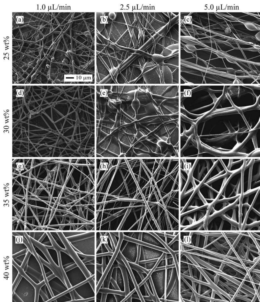
Fig. 3 SEM pictures ( \times 1\text{K} magnification) of SMP electrospun fibers with different PS solution concentrations of 25 wt % (a–c), 30 wt % (d–f), 35 wt % (g–i) and 40 wt % (j–l) at various flow rates of 1.0 \mu\text{L min}^{-1} (a, d, g, j), 2.5 \mu\text{L min}^{-1} (b, e, h, k) and 5.0 \mu\text{L min}^{-1} (c, f, i, l).
