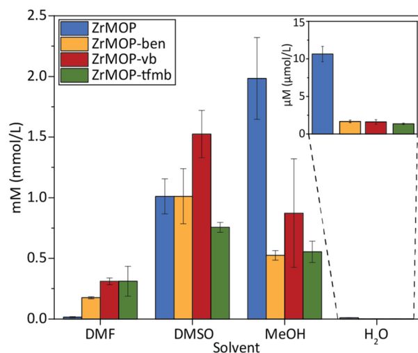
Fig. 5 Graphical representation of the solubility of ZrMOP and functionalized analogues in dimethylformamide (DMF), dimethyl sulfoxide (DMSO), methanol (MeOH), and water ( \text{H}_2\text{O} ).
