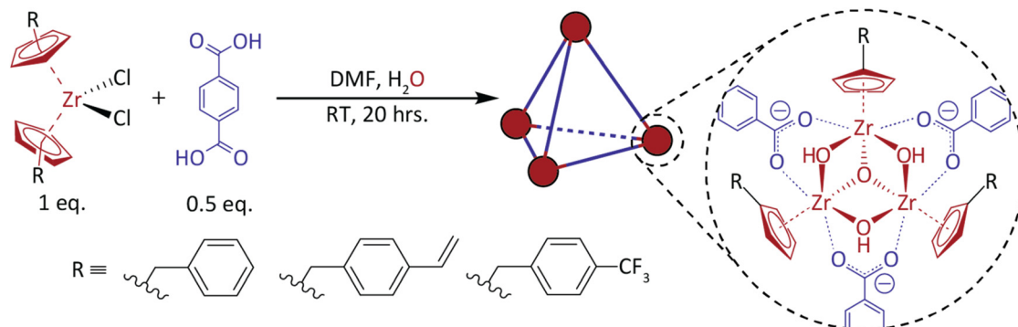
Fig. 1 Synthesis of functionalized ZrMOPs .
