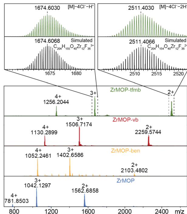
Fig. 3 Stacked high resolution mass spectra of ZrMOP and functionalized analogues, with simulated and experimental isotope patterns of ZrMOP-tfmb 2+ and 3+ charge states.
