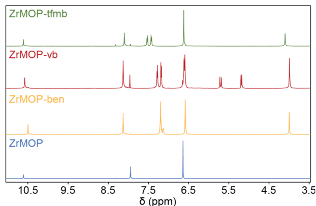
Fig. 2 Stacked ^1\text{H} NMR spectra of ZrMOP and functionalized analogues, in \text{DMSO}-d_6 at room temperature.
