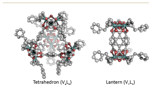
Fig. 4 Crystal structures of ZrMOP-ben tetrahedron and lantern architectures.
