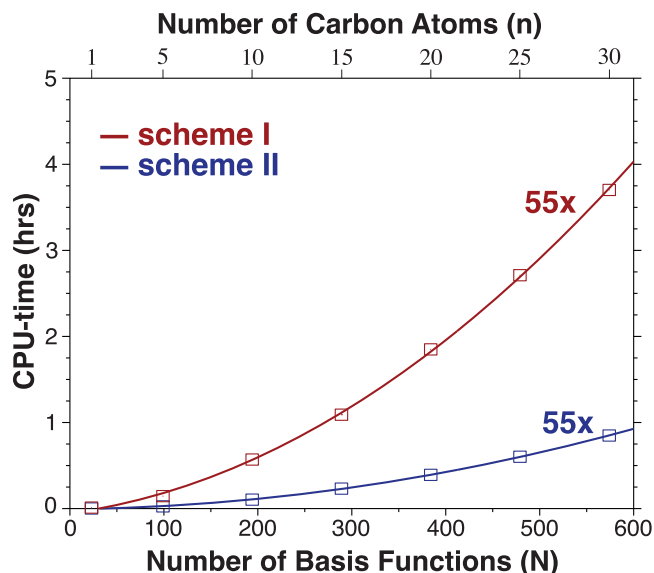
Figure 1. Timing benchmarks as a function of basis set ( N ) and increasing chain length ( n ) for a series of alkane molecules. The timings reported are the full evaluation of the set of analytic nuclear gradient and first-order derivative coupling vectors (55 in total). The ten lowest-energy singlet excited states of each system were included. The red curve (scheme I) and the blue curve (scheme II) corresponds to a polynomial least-squares fit.
