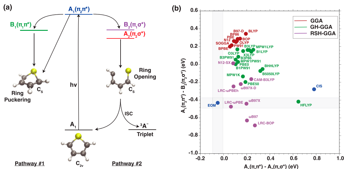
Figure 5. (a) A simplified schematic of the available nonadiabatic pathways to ring opening and ring puckering in selenophene. (b) Energy differences between the A_1(\pi_2\pi^*) , A_2(\pi_2\sigma^*) , and B_2(\pi_1\sigma^*) excitation energies referenced from the C_{2v} geometry on the ground electronic state for each method. The EOM-EE-CCSD results are shown in blue for reference.
