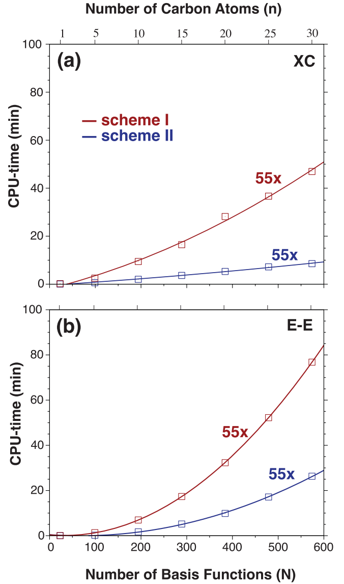
Figure A1. Timing data as a function of basis set size and increasing chain length for the exchange-correlation (XC) integral derivative contractions (a) and the electron-electron (E-E) repulsion integral derivative contractions (b). The red curves (scheme I) and the blue curves (scheme II) correspond to a polynomial least-squares fit of the timings of each component.
