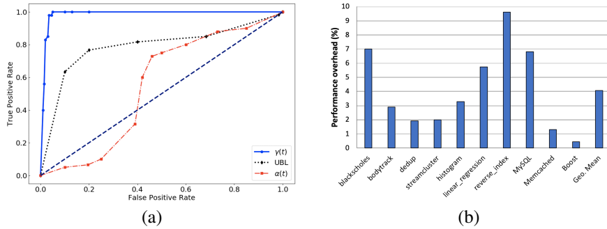
Figure 6: (a) Effect of error threshold, (b) Profiling overhead.
