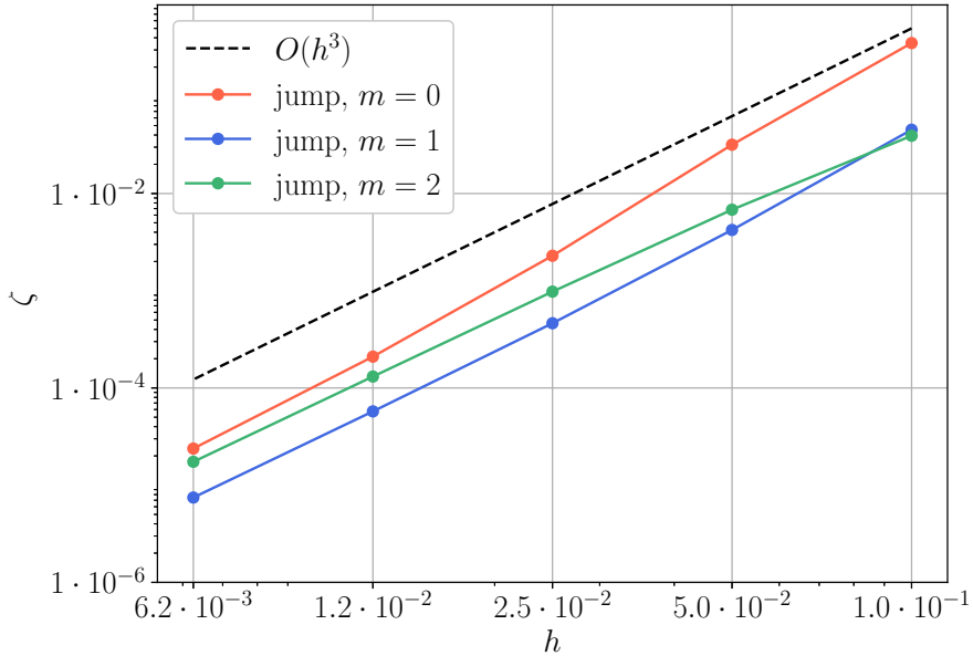
Figure 5. Order of convergence of \mathbf{L}^2 relative errors in magnetic field with jump in electrical current with respect to mesh size h . The dash line represents the theoretical order of convergence h^3 .
