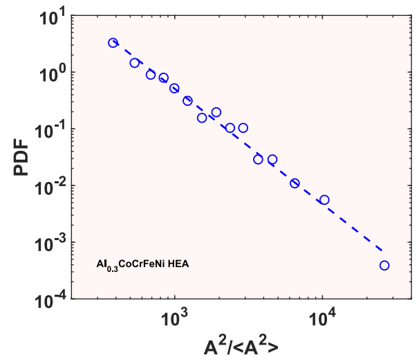
Fig. 11. Power-law statistics of the AE. The log-log plot of the PDF for the normalized intensity of the AE, A^2/\langle A^2 \rangle , for a sample tested at 10^{-3} \text{ s}^{-1} . The analyzed dataset contained 392 hits. The dashed line corresponds to an exponent, \beta = 2.1 \pm 0.1 .
