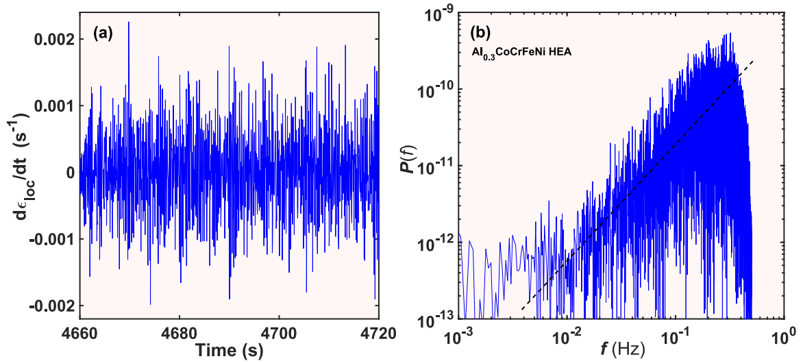
Fig. 8. Example of the local strain-rate response. (a) The detrended signal for the local d\epsilon_{loc}/dt signal corresponding to the middle of the gage part of the sample tested at a strain rate of 10^{-5} \text{ s}^{-1} and (b) its power spectrum (cf. Fig. 3). The dashed line corresponds to the function of P(f) \sim f^{1.5} .
