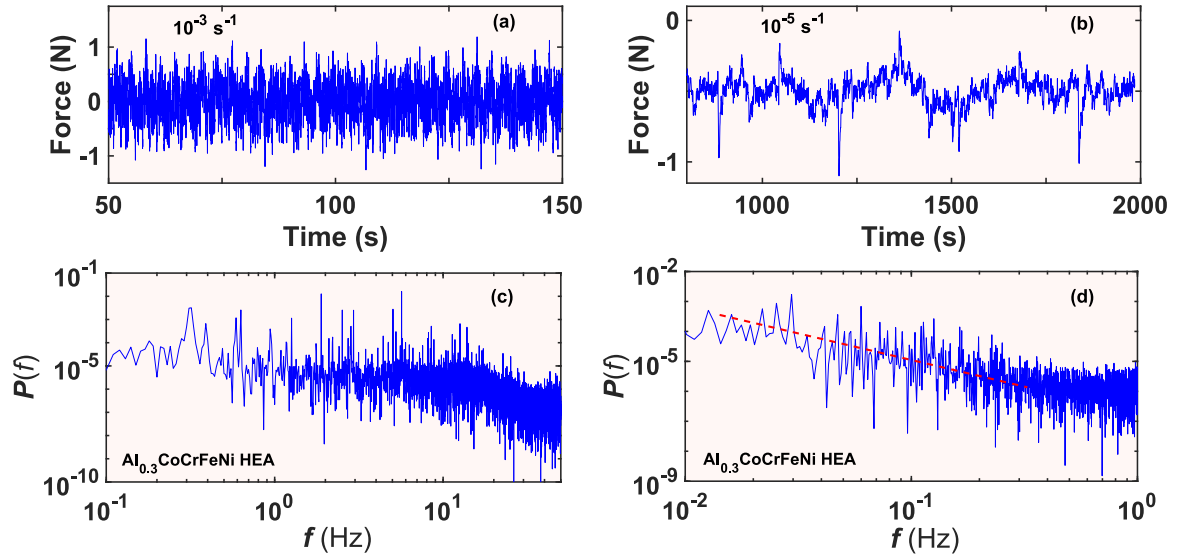
Fig. 3. Examples of the force response: detrended force vs. time signals for the samples tested at a strain rate of (a) 10^{-3} \text{ s}^{-1} and (b) 10^{-5} \text{ s}^{-1} and the corresponding power spectra (c) and (d). The dashed line in (d) traces P(f) \sim 1/f^{1.8} .
