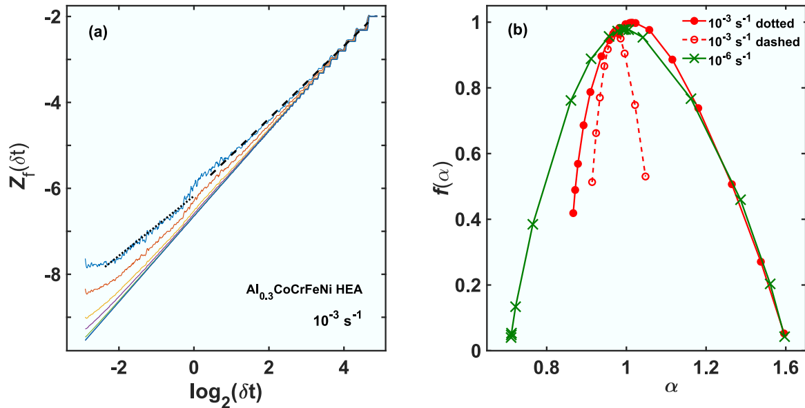
Fig. 7. Multifractal scaling for the force response. (a) Examples of the partition functions for the force signal corresponding to the sample tested at a strain rate of 10^{-3} \text{ s}^{-1} ; (b) the MF spectra for the intervals shown in chart (a) by the dotted and dashed lines (respectively, solid and open circles), as well as for the strain rate of 10^{-6} \text{ s}^{-1} (crosses).
