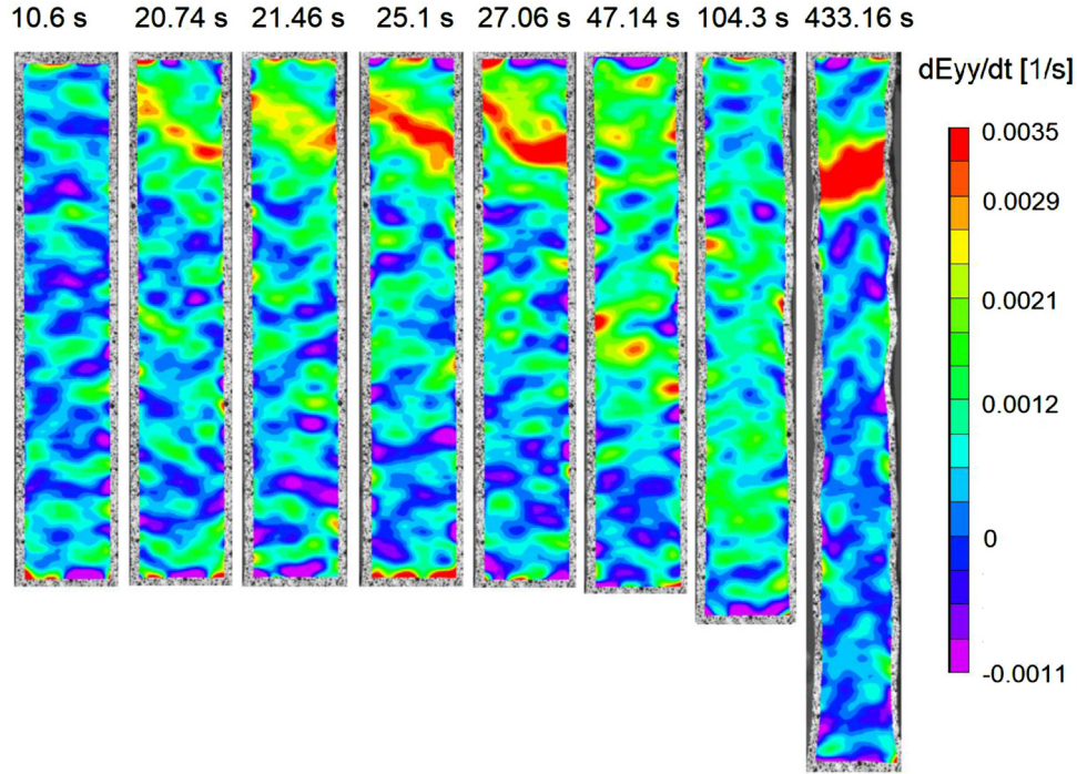
Fig. 2. The DIC for the \text{Al}_{0.3}\text{CoCrFeNi} HEA sample of Fig. 1. Images of the local strain-rate field are superposed onto the photographs of the gage part of the surface of the deforming sample, covered with a speckle pattern. It is worth noting the waviness of the borders of the heavily-deformed specimen in the last image. Green regions correspond to the strain rate around \dot{\epsilon}_a .
