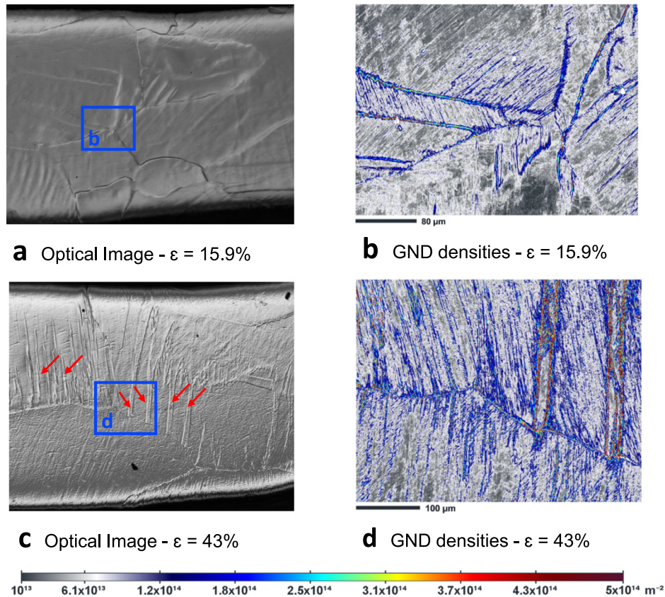
Fig. A1. Microstructures of the HEA samples deformed to strains of 15.9% and 43.3%. (a) and (c) - optical images. (b) and (d) - geometrically necessary dislocation (GND) densities for smaller regions approximately indicated on optical images. The grain boundaries in GND maps appear as black solid lines. Arrows indicate some of the twins presented in the microstructure.
