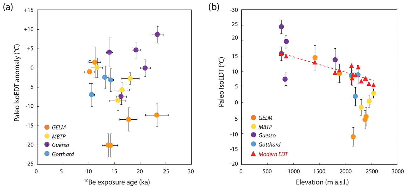
Figure 10. (a) Relationship between ^3\text{He} paleoIsoEDT anomaly and ^{10}\text{Be} exposure age from available data from moraine boulders and glacially scoured bedrock surfaces in the Alps (results from this study; Tremblay et al., 2018, Gesso, and Guralnik et al., 2018, Gotthard). (b) Relationship between ^3\text{He} paleoIsoEDT and elevation for same dataset as in panel (a).
