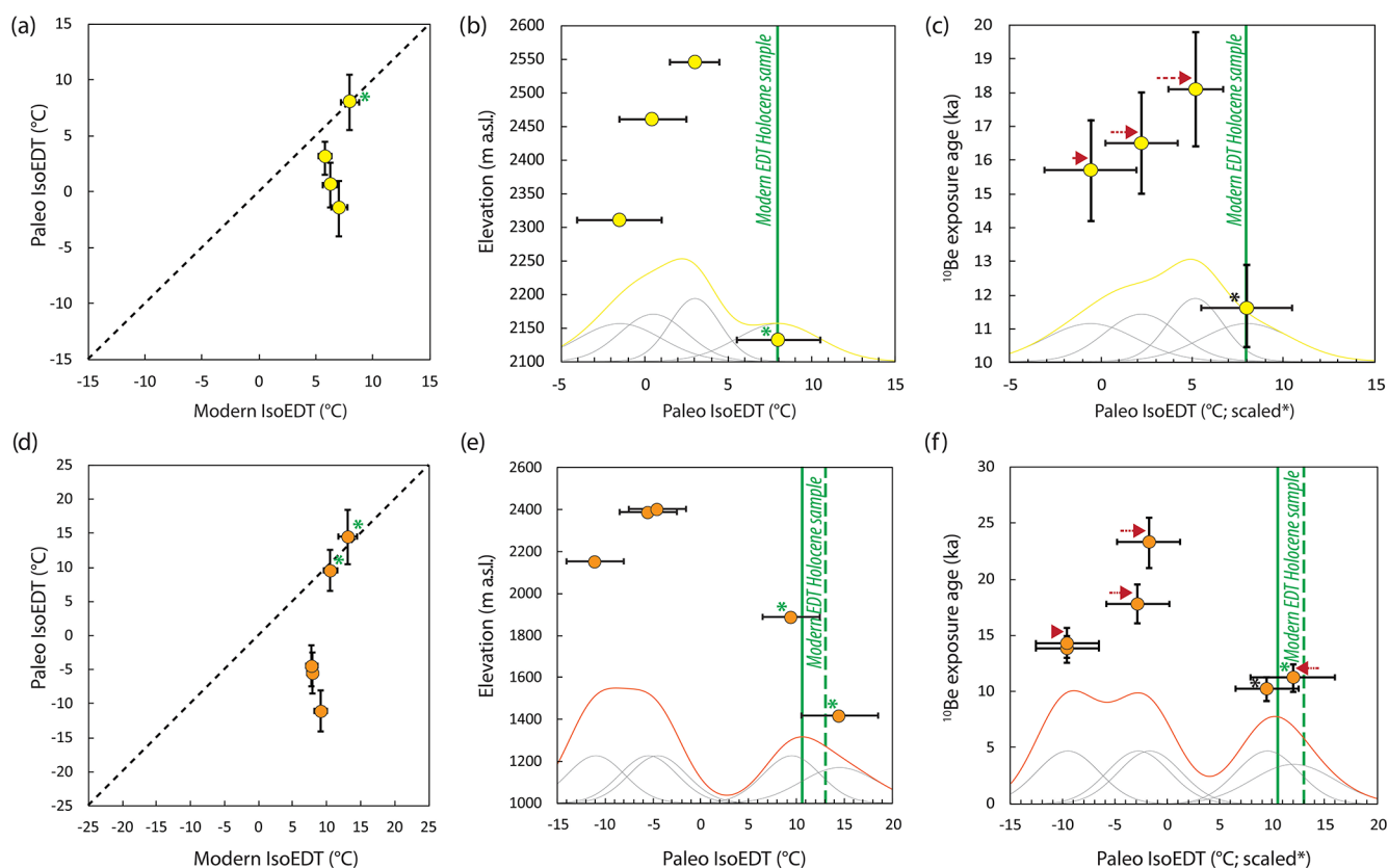
Figure 5. Distribution of ^3\text{He} -derived paleoIsoEDTs along the MBTP (a–c) and GELM (d–f) deglaciation profiles. Holocene samples used for calibration are marked by asterisks. (a, d) PaleIsoEDTs relative to modern EDTs (black dashed line is 1 : 1); (b, e) relationship between paleIsoEDT and elevation; and (c, f) relationship between paleIsoEDT and ^{10}\text{Be} exposure age after correction for lapse rate (marked by red arrows, relative to the Holocene sample marked with a black asterisk). Green solid and dashed lines are modern EDTs for Holocene samples, with the solid line indicating the modern EDT taken as reference for the lapse rate correction. The thin lines represent the sums (yellow and orange) of the individual (gray) probability distributions of paleoIsoEDTs.
