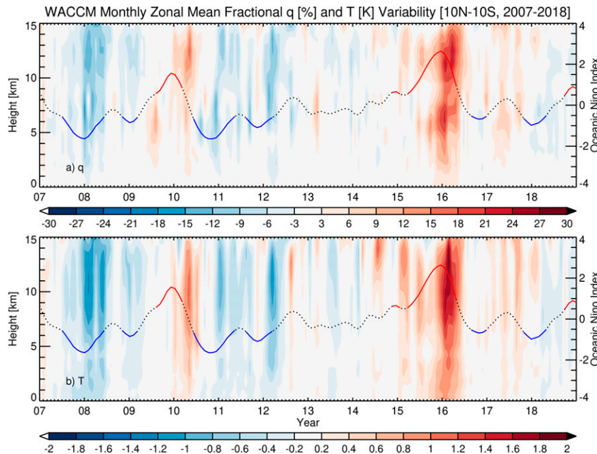
FIG. 6. Time–height cross sections of WACCM monthly zonal mean (a) fractional specific humidity (%) and (b) temperature (K) variability from 2007 to 2018 within 10^{\circ}\text{N} – 10^{\circ}\text{S} . The ONI is also shown, as in Fig. 4.
