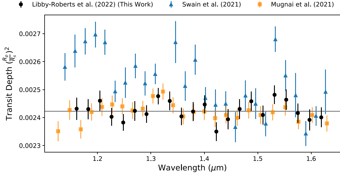
Figure 10. A comparison between the average transit depths in Swain et al. (2021) (blue/triangle points), in Mugnai et al. (2021) (orange/square points), and in this work (black/circle points). All utilize the same HST/WFC3 data, though Swain et al. (2021) determine very different transit depths, most notably at shorter wavelengths. Transit depths derived in this work and in Mugnai et al. (2021) are statistically the same, with similar uncertainties as well.
