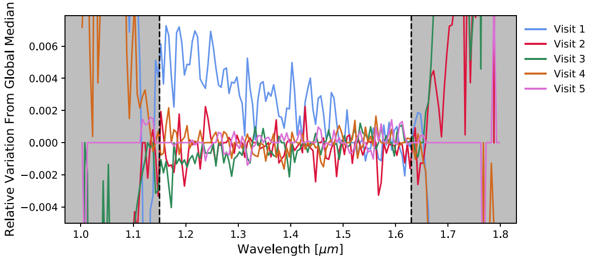
Figure 2. The deviation of each visit from the global medium-combined stellar spectrum created from the combination of all five visits. Visits 2–5 show <0.2\% difference across 1.15\ \mu\text{m} and 1.63\ \mu\text{m} , while Visit 1 differs by <0.8\% , most notably at shorter wavelengths. Dashed lines highlight the high-S/N region.
