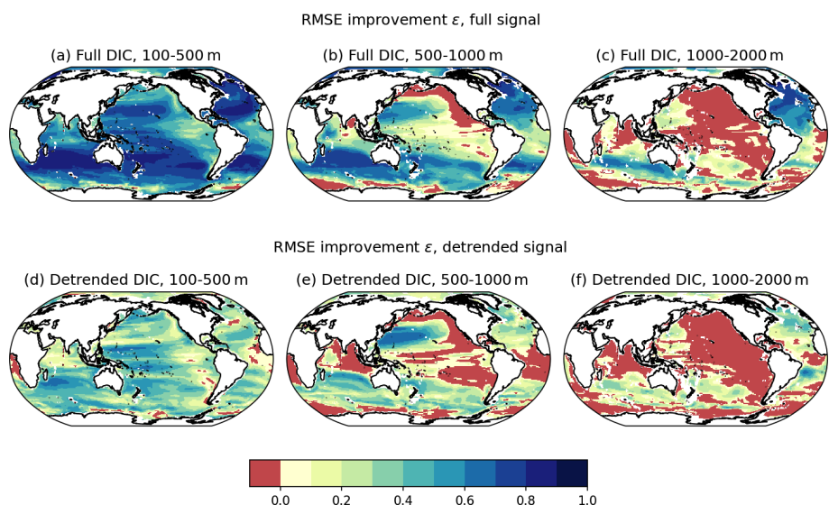
Figure 8. Average RMSE reduction \varepsilon , relative to a climatology, for sensitivity tests with out-of-sample models: panels ( a–c ) use average \varepsilon for the full DIC' signal and panels ( d–f ) use average \varepsilon for the detrended signal. The average RMSE reduction is calculated for individual depth levels: 100–500 m ( a, d ), 500–1000 m ( b, e ), and 1000–2000 m ( c, f ).
