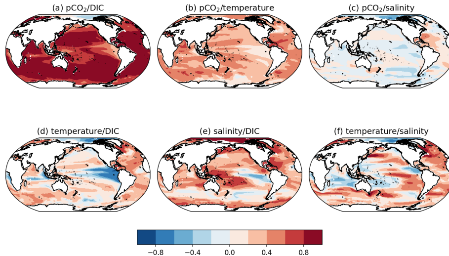
Figure 2. Correlations for the entire CMIP6 historical ensemble between changes in (a) atmospheric p\text{CO}_2 and upper-ocean (0–100 m integrated) DIC, (b) atmospheric p\text{CO}_2 and upper-ocean temperature, (c) atmospheric p\text{CO}_2 and upper-ocean salinity, (d) upper-ocean temperature and DIC, (e) upper-ocean salinity and DIC, and (f) upper-ocean temperature and salinity.
