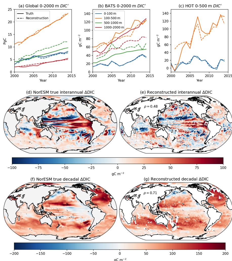
Figure 9. Reconstructions of NorESM 0–2000 m carbon inventories. (a) Globally integrated NorESM carbon inventories (solid lines) and reconstructed carbon inventories using temporally varying Argo coverage (dashed lines; Pg C). Colours indicate depths: 0–100 m (blue), 100–500 m (orange), 500–1000 m (green), and 1000–2000 m (red). (b) As for panel (a) but with vertically integrated DIC concentrations at BATS ( \text{gC m}^{-2} ). (c) As for panel (b) but with vertically integrated DIC concentrations at HOT to 500 m ( \text{gC m}^{-2} ). Snapshots of inter-annual changes in 0–2000 m DIC ( \text{gC m}^{-2} ): (d) NorESM truth and (e) reconstruction. Inter-annual changes are taken as the difference between year 2013 and year 2014 carbon fields. Snapshot of near-decadal changes in 0–2000 m DIC between periods 2001–2006 and 2009–2014 ( \text{gC m}^{-2} ): (f) NorESM truth and (g) reconstruction.
