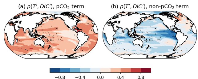
Figure 3. Breakdown of the correlation between upper-ocean DIC and temperature, \rho(\text{DIC}', T') , from Fig. 2d: (a) a term proportional to the variance of atmospheric p\text{CO}_2 and (b) a term consisting of the covariance of the residuals calculated after removing a linear fit against atmospheric p\text{CO}_2 . For a discussion of the breakdown of the correlation into terms and of the approximation, see Appendix A.
