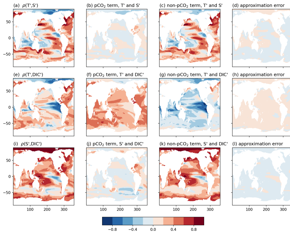
Figure A1. Correlation fields between non- p\text{CO}_2 variables T' , S' , and \text{DIC}' , with their terms from Eq. (A5) and approximation errors to measure the level of mismatch between Eqs. (A4) and (A5).
