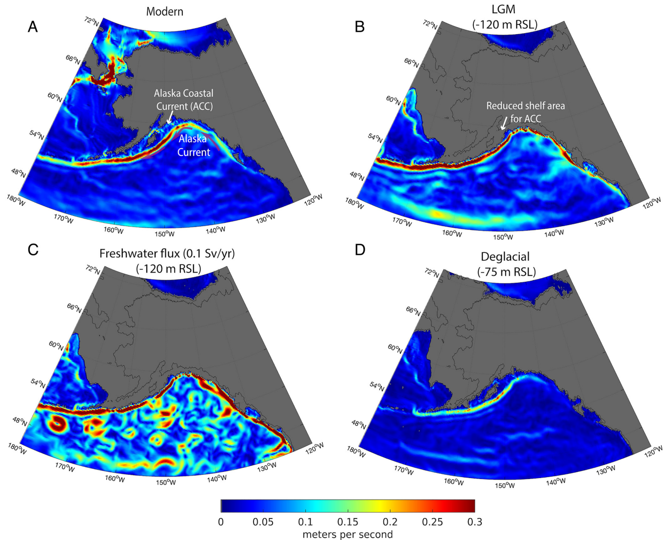
Fig. 2. Simulations of ocean currents in the Northeast Pacific under different climate and sea level conditions: Modern climate state (A), LGM climate state, with sea level \sim 120 m below modern (B), LGM boundary conditions with an increased freshwater flux (C), and intermediate sea level ( \sim 75 m), as would have occurred during the mid-deglacial period (D). Mean annual surface ocean velocity shows a strengthening of the cyclonic Alaska Current during the LGM relative to modern conditions, as well as a contraction of the shelf area on which the ACC flows. Boundary currents flow in a cyclonic (anticlockwise) direction.
