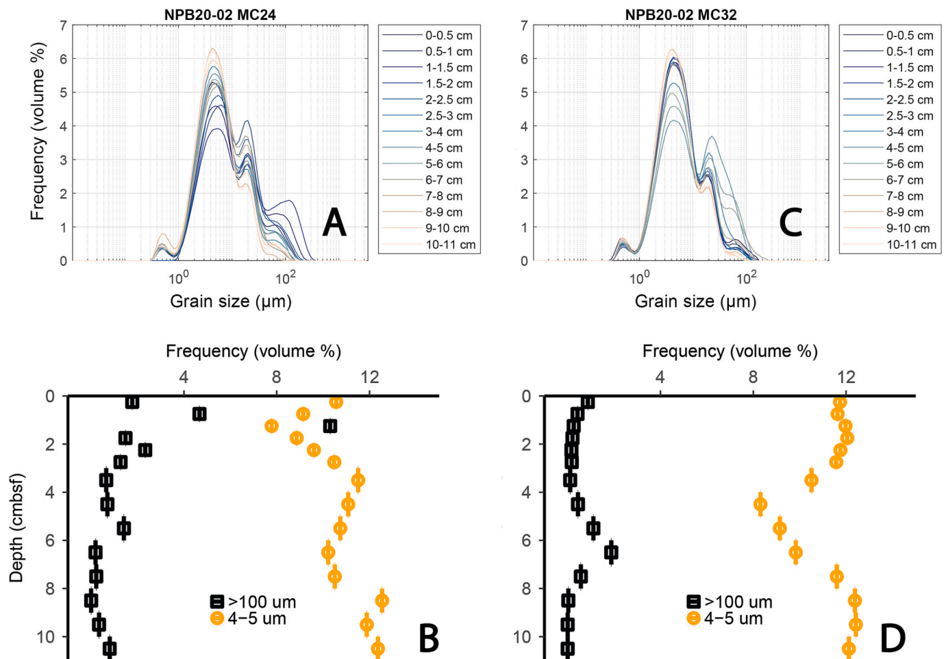
Fig. 4. Frequency distribution of grain size ( \mu\text{m} ) plotted on a log axis at the Pine Island (A) and Thwaites (C) sites, with the color of the line indicating the depth in the sediment (warmer colors = deeper, cooler colors = shallower). Depth profiles of the 4–5 \mu\text{m} (orange circles) and > 100 \mu\text{m} (black squares) grain size fractions at the Pine Island (B) and Thwaites (D) sites. Vertical bars indicate the depth interval over which each sediment sample was homogenized.
