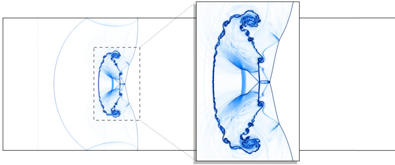
Fig. 4. Schlieren plots for the shock-bubble interaction benchmark for t = 40 \mu s .
