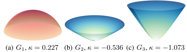
Figure 2: Illustration of the Riemannian spaces in the task graphs G_t on ogbn-arXiv. \kappa is the learnt curvature.
