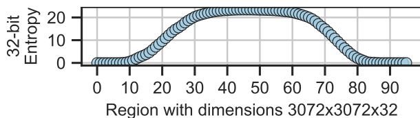
Fig. 7: The 32-bit Entropy for each 3072x3072x32 region of the 3072x3072x3072 Density object in the Miranda dataset. The x-axis is the region number in the z-dimension.
