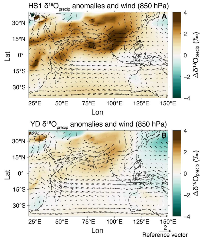
Fig. 4. Simulated summer (June to August) \delta^{18}\text{O}_{\text{precip}} anomalies and wind (850 hPa). (A) HS1 and (B) YD relative to BA in response to MWF in iTRACE. The wind field in (A) and (B) represent mean conditions during HS1 and YD, respectively. Coastlines (black outline) for HS1 and YD correspond to 120- and 60-m drop in sea level, respectively.
