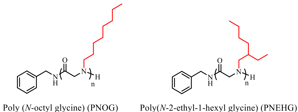
Scheme 1. Chemical structures of PNOG and PNEHG
