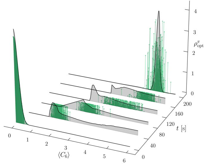
Fig. 7: Snapshots of the optimally controlled joint PDFs \rho_{opt}^\pi steering the state \langle C_6 \rangle distribution from the given \rho_0 to \rho_T , as in Fig. 1, over the given time horizon [0, T] \equiv [0, 200] s subject to the controlled noisy nonlinear sample path dynamics (1). The solid black curves with grey filled areas are obtained from the PINN. The stem plots are the KDE approximants of the optimally controlled PDF snapshots obtained from the closed-loop sample paths, as explained in Sec. V.
