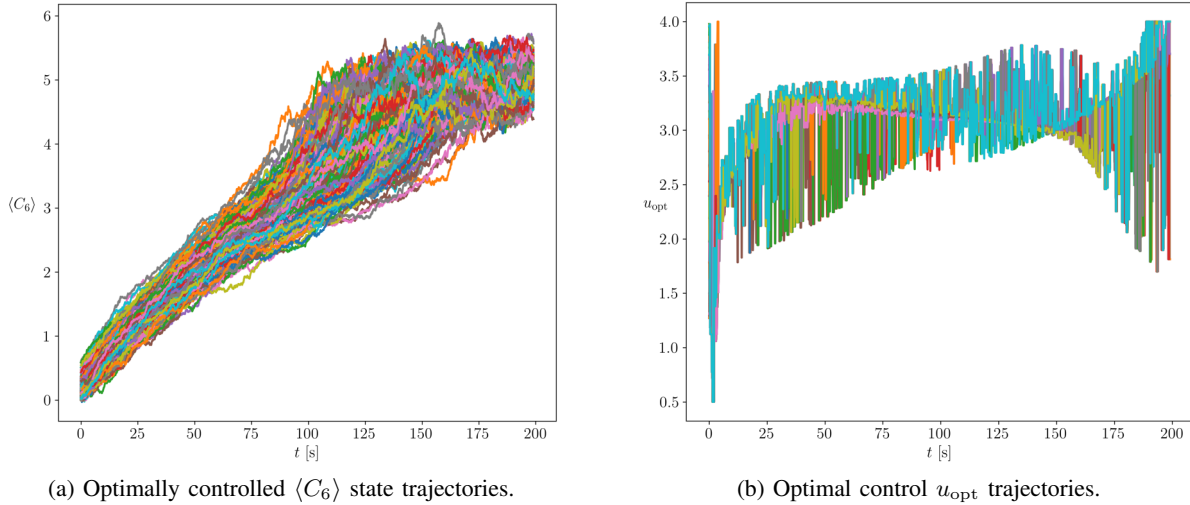
Fig. 8: The 1000 random sample paths resulting from the closed loop simulation using the learnt optimal policy \pi_{opt}(\langle C_6 \rangle, t) .
