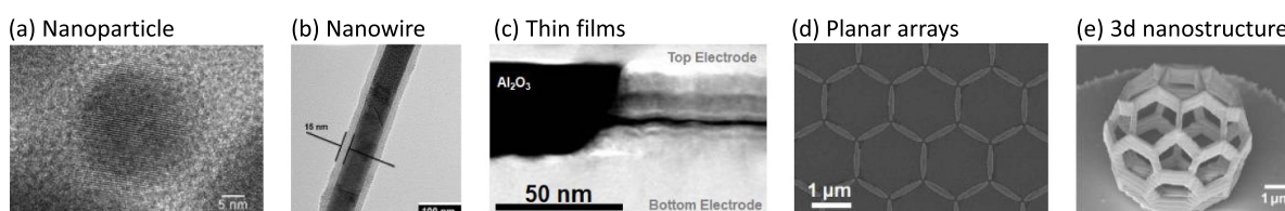
Figure 10. Selection of geometries studied in nanomagnetism: (a) nanoparticle of \text{Gd}_5(\text{Si}, \text{Ge})_4 used in magnetocaloric applications; (b) oxide-shell-protected \text{Mn}_5\text{Si}_3 nanowire. Reproduced from [75] with permission from the Royal Society of Chemistry. (c) Multi-layered thin-films stack of a \text{MgO} -based MTJ used in a nanosensor device. Reproduced from [71]. © IOP Publishing Ltd. All rights reserved. (d) Kagome Ni spin-ice array; (e) co-coated artificial buckyball used for x-ray tomography demonstration. Reprinted (figure) with permission from [76], Copyright (2015) by the American Physical Society.
