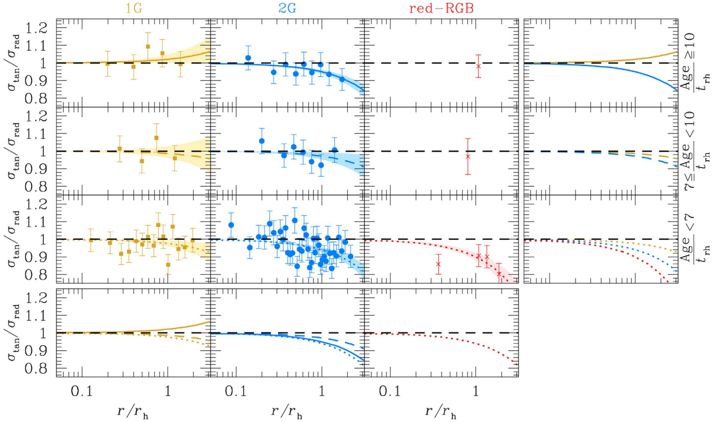
Figure 3. As in the left panels of Figure 2, but dividing the sample of GCs according to their dynamical age (age/ t_h ratio). The first three columns show the anisotropy for 1G (gold squares), 2G (blue dots), and red-RGB (red crosses), respectively. The black, horizontal lines mark the isotropic case. The lines, colored as the point in the same plot, are a straight-line fit to the data (see details in Figure 2; no line was fit for the red-RGB samples with only one data point). The first three rows present the result for old, intermediate, and young GCs, from top to bottom, respectively. The rightmost panels collect the straight-line fits for each population for GCs with the same dynamical age, while the panels at the bottom show the comparison between the trends of each mPOP in clusters with different dynamical ages.
