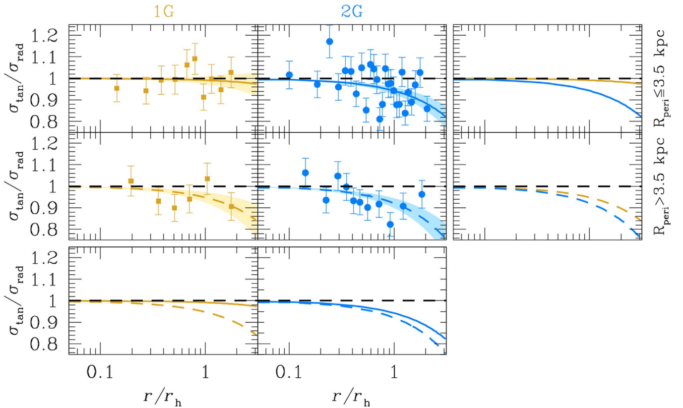
Figure 4. Similarly to Figure 3, we show the anisotropy as a function of distance from the centers of the clusters in units of r_h for mPOPs in clusters with different R_{\text{peri}} . The top and middle rows present the 1G (gold) and 2G (blue) anisotropy profiles for GCs with R_{\text{peri}} \leq 3.5 kpc and R_{\text{peri}} > 3.5 kpc, respectively. The black, horizontal line is set to 1 (isotropic case). The colored lines are a straight-line fit to the data (see details in Figure 2). The comparison between the straight-line fit for mPOPs in GCs with the same R_{\text{peri}} is given in the rightmost panels, while between the same mPOP in GCs with different R_{\text{peri}} is highlighted in the bottom panels.
