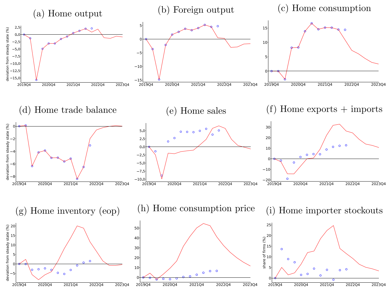
Fig. 15. Endogenous variables.
