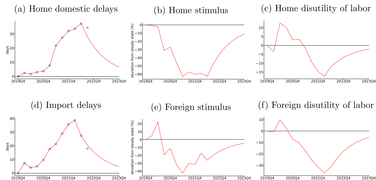
Fig. 14. Exogenous shocks.
