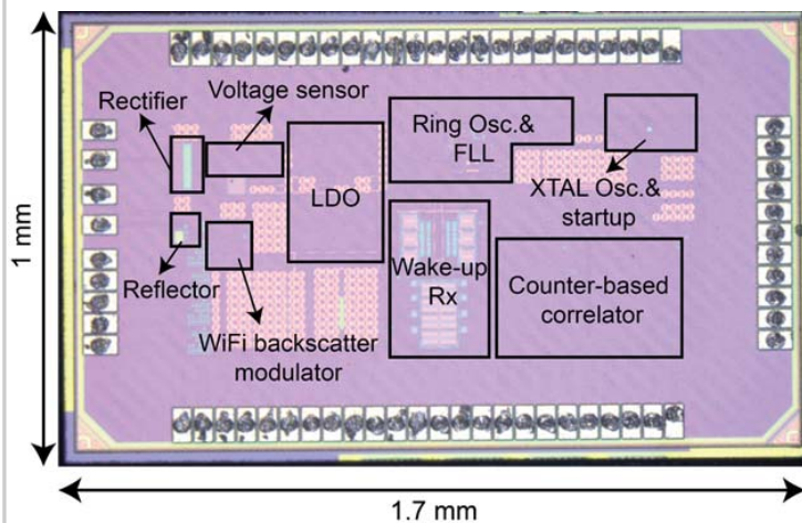
Figure 21.5.7: Die micrograph of the proposed single-device-interrogated LTE-powered BLE-to-WiFi backscattering chip.
