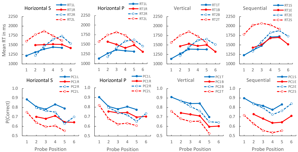
Fig. 3. Probe Position Effects Experiments 1–4. Note: Mean response time (RT; top row) and accuracy (P(Correct); bottom row) for first (solid lines) and second (dashed lines) responses in forward (L before R, T before B, S before E = blue) and backward (R before L, B before T, E before S = red) cue orders in Experiments 1–4 as a function of probe position. L, R (horizontal), T, B (vertical), and S, E (sequential) refer to the relative positions of the cues in the list. (For interpretation of the references to colour in this figure legend, the reader is referred to the web version of this article.)
