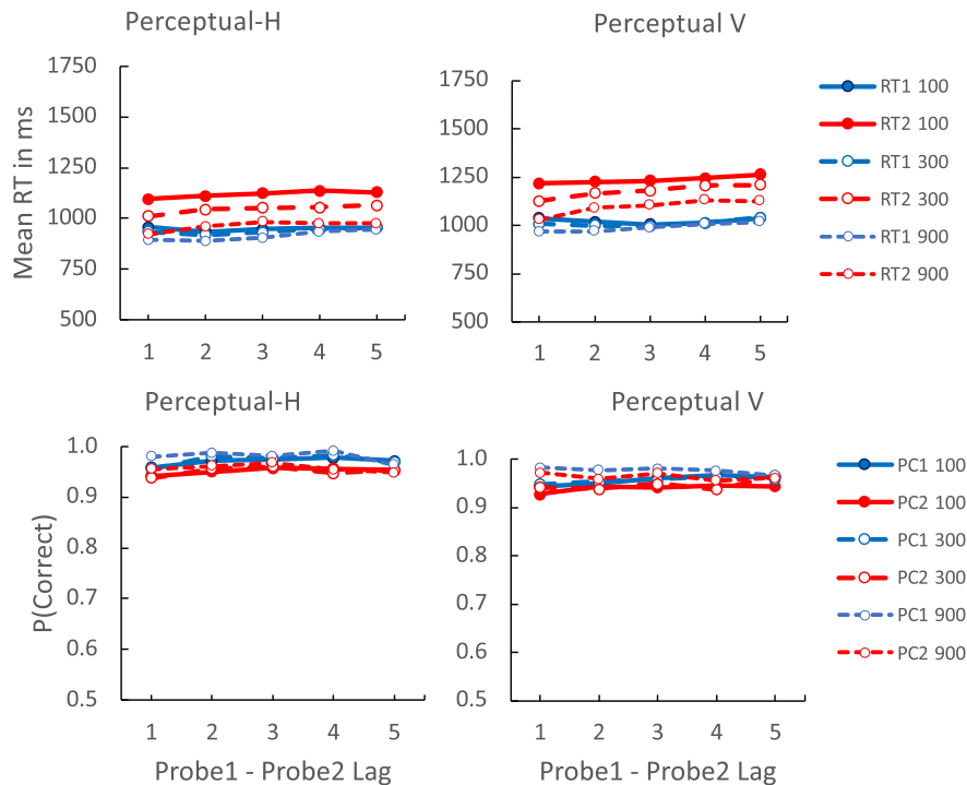
Fig. D2. SOA \times Lag Experiments 5–6. Note: Interactions between stimulus onset asynchrony (SOA = 100, 300, 900 ms) and response (RT1 vs. RT2) as a function of lag between the first and second probes in Experiments 5–6. Top row: RT; bottom row: accuracy.
