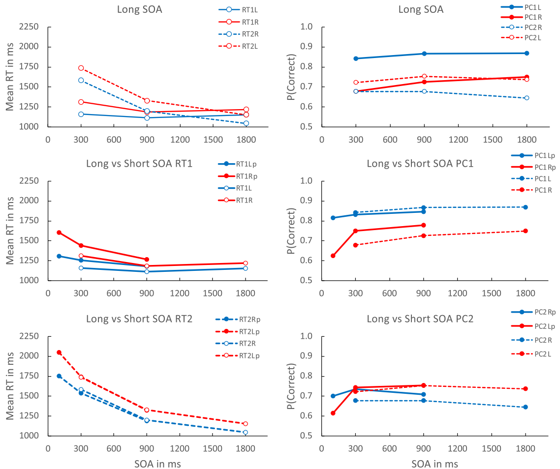
Fig. B1. SOA Effects with Long SOAs. Note: Response time (RT; left panels) and accuracy (P(Correct); right panels) as a function of stimulus onset asynchrony (SOA) and direction ( forward = L then R = blue; backward = R then L = red) in the long SOA experiment. L and R refer to the relative positions of the cues in the list. The top row shows RT1 and RT2 (left) and PC1 and PC2 (right panel) as a function of SOA. The middle row compares RT1 and PC1 from the long SOA experiment with data from a short SOA experiment (Experiment 2: Horizontal P). Slowing is apparent in the RT1 data. The bottom row compares RT2 and PC2 from the long SOA experiment with data from the short SOA experiment (Experiment 2).
