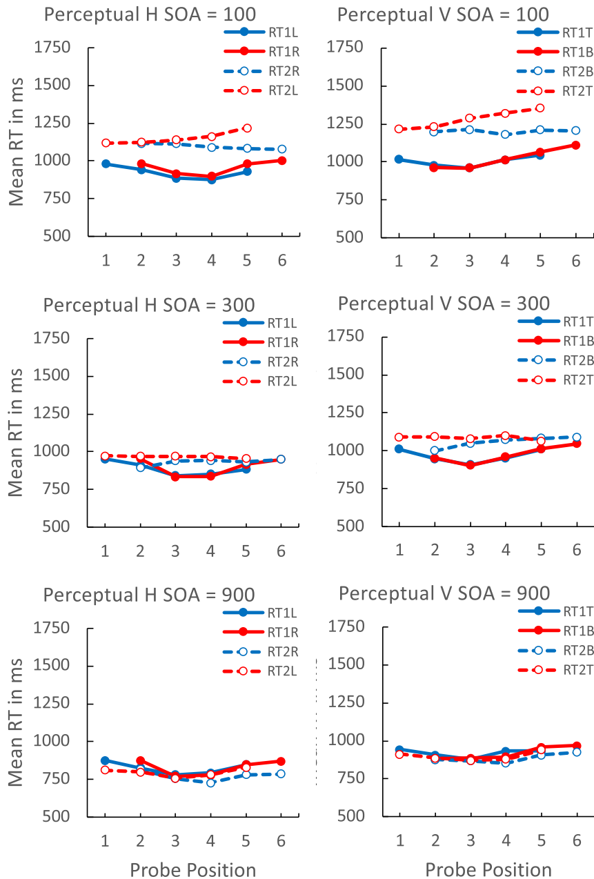
Fig. C2. Position \times Direction at Each SOA Experiments 5–6. Note: Interactions between direction ( forward = L then R = blue; backward = R then L = red) and response (RT1 vs. RT2) as a function of probe position in Experiments 5–6. L, R (horizontal), T, B (vertical), and S, E (sequential) refer to the relative positions of the cues in the list. Top, middle, and bottom rows present data from stimulus onset asynchrony (SOA) = 100, 300, and 900 ms, respectively.
