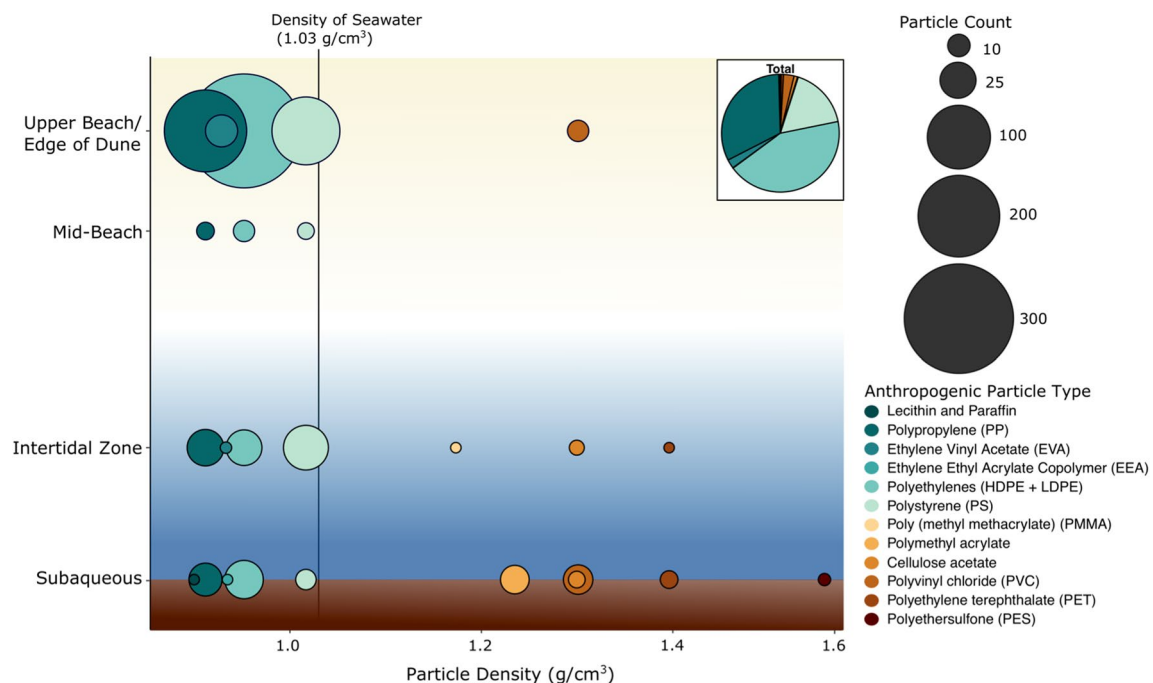
Figure 3. Abundance of microplastic particle types varied between sampling zones (e.g., upper beach, mid-beach, intertidal zone, subaqueous). The size of the dot represents the microplastic particle count. The color represents both the particle type and the corresponding particle density. Particles less dense than seawater ( < 1.03 \text{ g cm}^{-3} ) are shown in green and blue shades. Particles more dense than seawater ( > 1.03 \text{ g cm}^{-3} ) are shown in shades of brown. For polymers with a range of possible densities (e.g., polystyrene), the average density was used. The overall frequency for all sites and sampling zones is shown in the “Total” pie chart in the top righthand corner.
