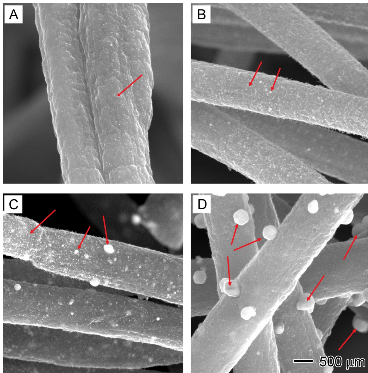
Figure 8. SEM images showing the nanoparticle growth on \frac{1}{2} Ni/Co nanofiber catalysts by increasing the heating temperature: (A) 450 °C, (B) 850 °C, (C) 1050 °C, and (D) 1250 °C.
