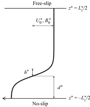
Figure 1. Initial mean profile for buoyancy and velocity showing dimensional parameters and boundary conditions. The bottom boundary moves to the left with speed -U_0^* \tanh(d^*/h^*) for computational efficiency.
