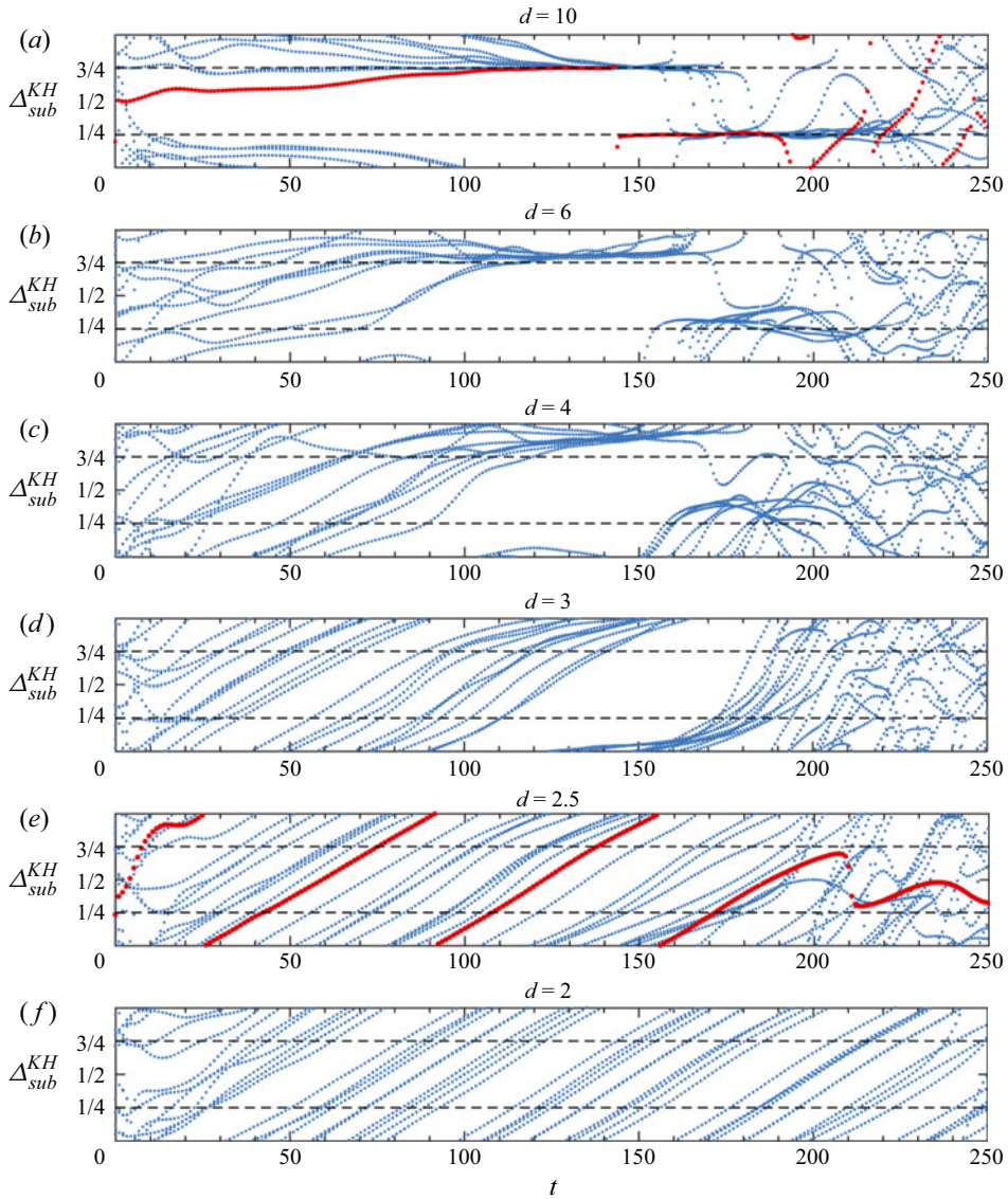
Figure 8. Time variations of \Delta_{sub}^{KH} with different values of d . Two horizontal dashed lines in each panel denote the optimal lock-on value, \Delta_{sub}^{KH} = 3/4 , and the opposite of optimal value, \Delta_{sub}^{KH} = 1/4 , respectively. Red curves indicate the cases selected in figure 7.
