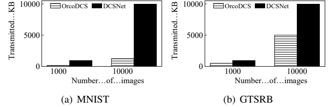
Fig. 3. Transmission cost for OrcoDCS and DCSNet. OrcoDCS can save up to 10\times transmission cost than DCSNet.
