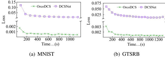
Fig. 4. Breakdown of time-to-loss performance. OrcoDCS can achieve lower loss faster than DCSNet in terms of training time.
