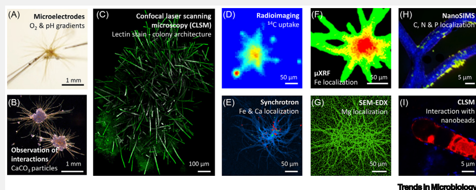
Figure I. Examples of experimental techniques used to analyze structure, composition, behavior, and physiology of Trichodesmium colonies. We acknowledge contributions from our collaborators: N. Kessler and M. Fine (panel B), T. Neu and U. Kuhllicke (panel C), S. Basu, S. Wang, and D. de Beer (panel D), S. Myneri, N. Kessler, R. Sanders, and D. Schlesinger (panel E), A.-N. Visser, F. Zhang, O. Qafoku, and R. Boiteau (panel G), A. Mijovilovich, H. Kuepper, A. Colussi, G. Konert, and O. Prášil (panel F), M. Kienhuis, R. Lopez Adams, and L. Polerecky (panel H), G. Konert (panel I). Abbreviations: µXRF, MicroXRF (micro-X-ray fluorescence analysis); nanoSIMS, nanoscale secondary ion mass spectrometry.
