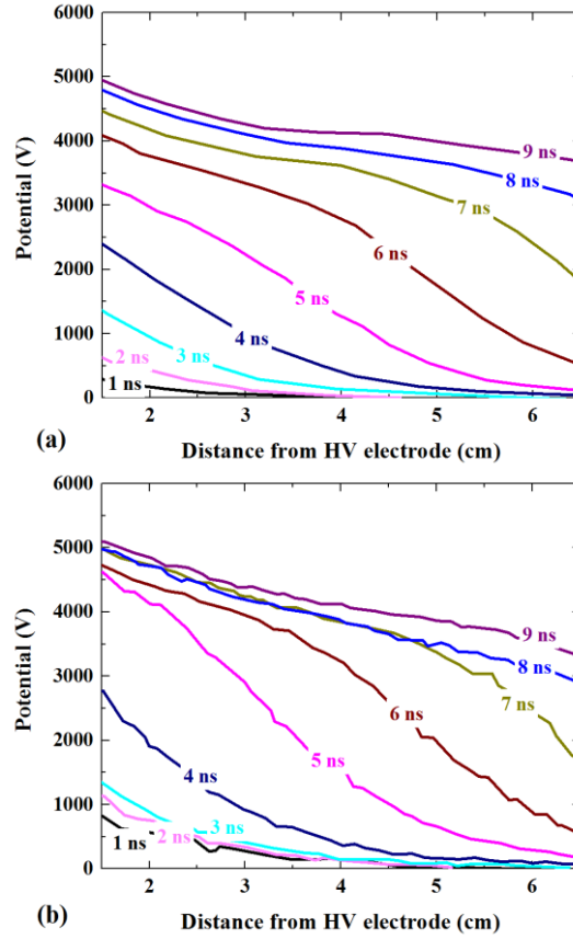
Figure 4. Validation of the axial potential profiles of the FIW during the propagation stage. Results were collected from the position of the tip of a capacitive probe, r = 1.27 \text{ cm} . (a) Model predictions. (b) Experimental measurements.
