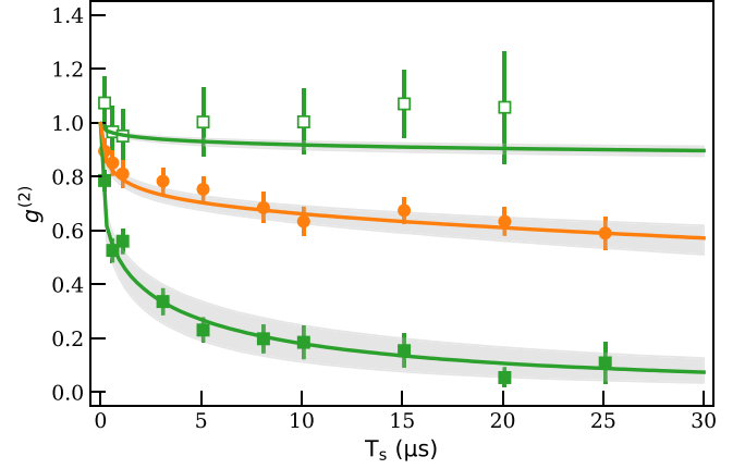
FIG. 2. Dynamic g^{(2)} as a function of interaction time T_s for varying interaction strength: (i) that with same atomic distribution \sigma_z = 10.5 \mu m but different principal quantum number n = 40 (orange closed circles) and n = 50 (green closed squares) and (ii) that with same principal quantum number n = 50 but different atomic distributions \sigma_z = 10.5 \mu m (green closed squares) and \sigma_z = 230 \mu m (green open squares). The solid line is the result of the numerical simulation together with 20% of \sigma_z (shaded area).
