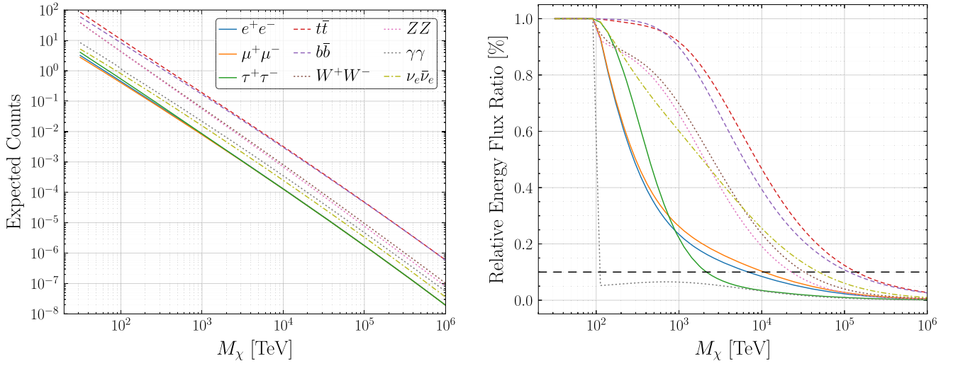
Figure 2. The number of expected \gamma -ray events (left) and relative ratio between the observable and total \gamma -ray energy flux (right). The expected counts are computed assuming an effective area of 10^{10} \text{ cm}^2 , 50 hr of exposure time, a J -factor of 10^{18} \text{ GeV}^2 \text{ cm}^{-5} \text{ sr}^{-1} , and \langle\sigma v\rangle = 10^{-23} \text{ cm}^3 \text{ s}^{-1} . The observable energy flux is defined as the integrated \gamma -ray energy flux up to 100 TeV, and for reference in the black dashed curve we show a value of 10%. The portion of the observable UHDM signal from M_\chi > 100 \text{ TeV} decreases progressively as M_\chi increases. The various line styles refer to the classes of annihilation channel: charged leptons (solid), quarks (dashed), gauge bosons (dotted), and \nu_e \bar{\nu}_e (dashed-dotted).
