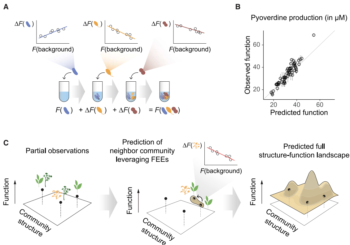
Figure 4. Global epistasis—like patterns in ecology—may help us infer the quantitative relationship between community composition and function
