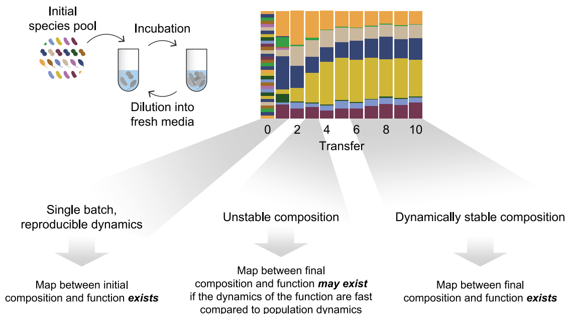
Figure 5. Conditions for the existence of an ecological structure-function map
