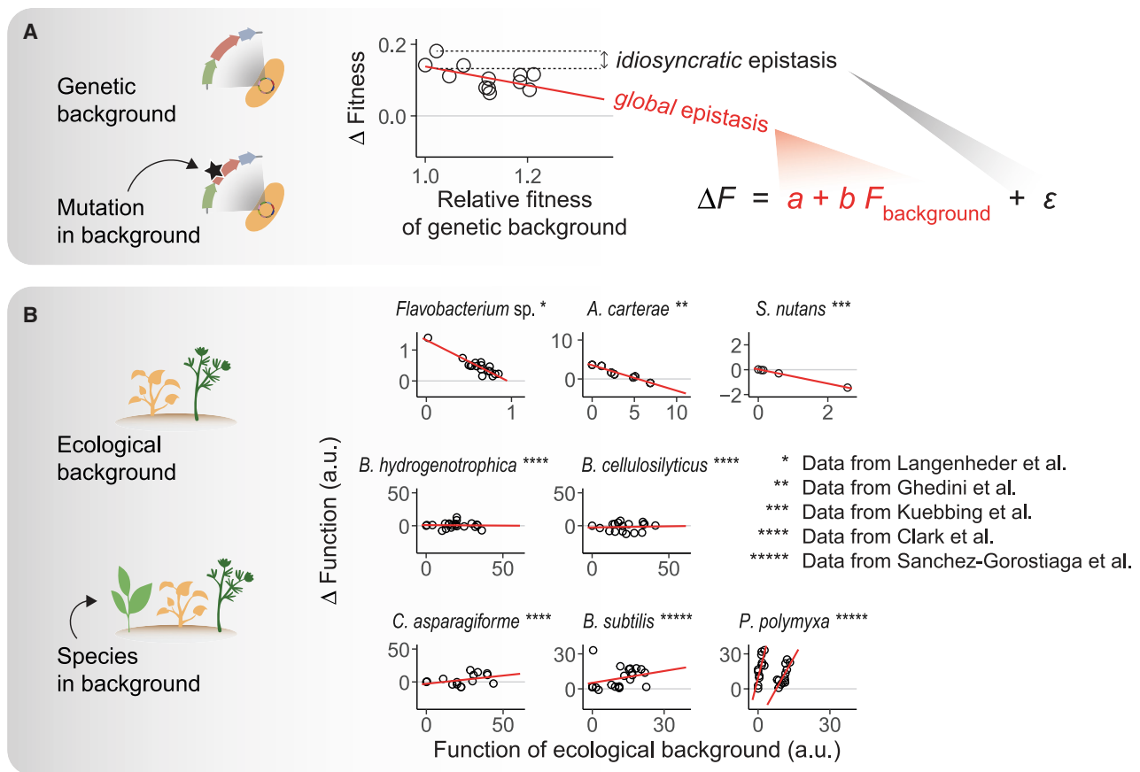
Figure 3. An analog to global epistasis explains the functional effect of adding new species to microbial consortia
