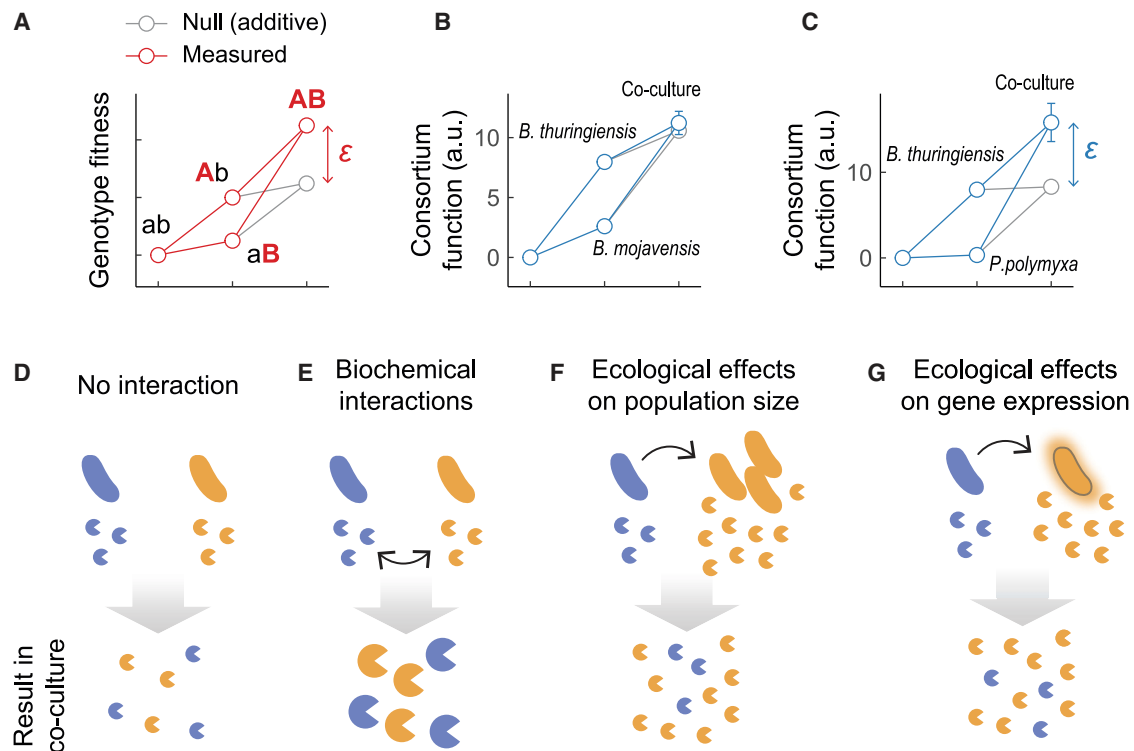
Figure 1. Species interactions create non-additive effects on community function
