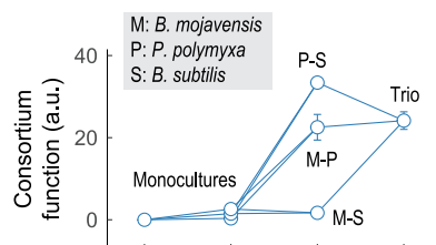
Figure 2. High-order functional interactions in microbial consortia
